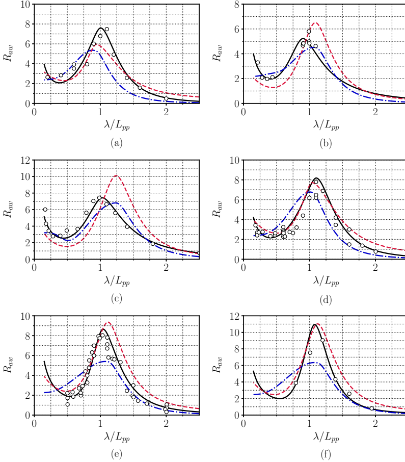
Figure 4.1: Added resistance in a regular head sea, \circ experimental data, — CTH, - - - ITTC-STA2, - - - NTUA; estimated for (a) Bulk carrier with F_n = 0.010 , (b) DTC container ship with F_n = 0.139 , (c) HSVA cruise ship with F_n = 0.232 , (d) KVLCC2 tanker with F_n = 0.142 , (e) S175 container ship with F_n = 0.200 , and (f) S.A. Van Der Stel with F_n = 0.250 .
