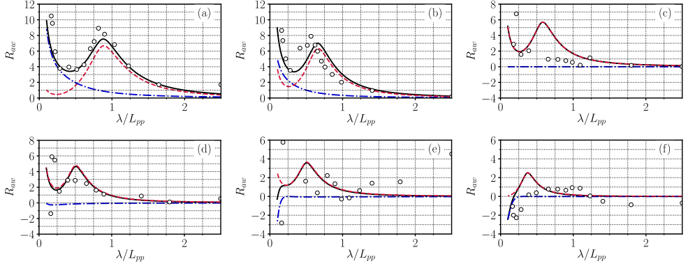
Figure 4.4: Added resistance for the HSVA cruise due to regular waves with arbitrary angles at F_n = 0.232 , \circ experimental data, — R_{aw} , - - - R_{awr} , ···· R_{awm} ; estimated at (a) 30 degrees, (b) 60 degrees, (c) 90 degrees, (d) 120 degrees, (e) 150 degrees, and (f) 180 degrees.
