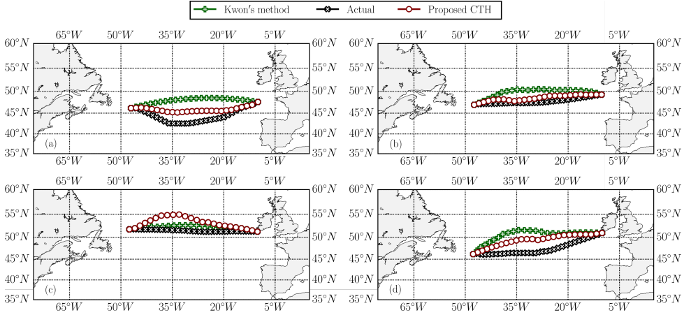
Figure 4.6: Optimal trajectories for the selected case study: (a) voyage 2009-01-18, (b) voyage 2009-02-18, (c) voyage 2009-12-26, and (d) voyage 2010-01-13.
