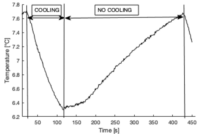
Fig. 1. Temperature variations in an RDC from Månsson and Ostermeyer (2019). When refrigeration is active, the temperature decreases from 7.7°C to 6.3°C within approximately 100 s. The temperature is then increasing back to the upper limit of 7.7°C for 300 s before the refrigeration cycle begins again.
