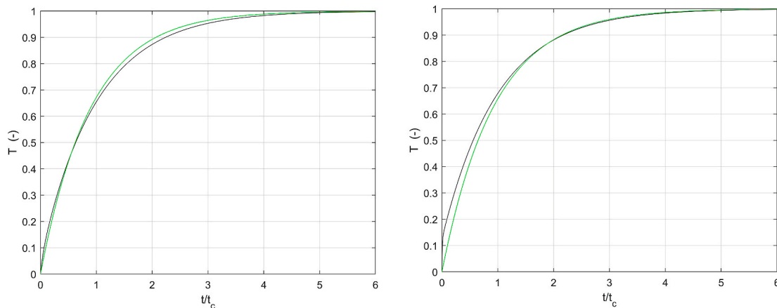
Fig. 26. Interior temperature response due to a step change in the interior heat source for Case III (left) and Case IV (right).
