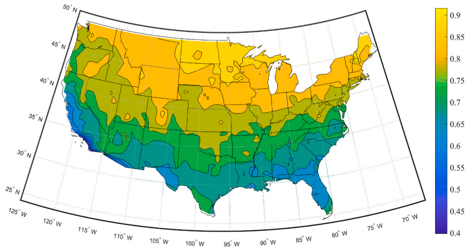
Fig. 20. \alpha for a prescribed Climate Zone 4A "Large Hotel" building across the U.S.
