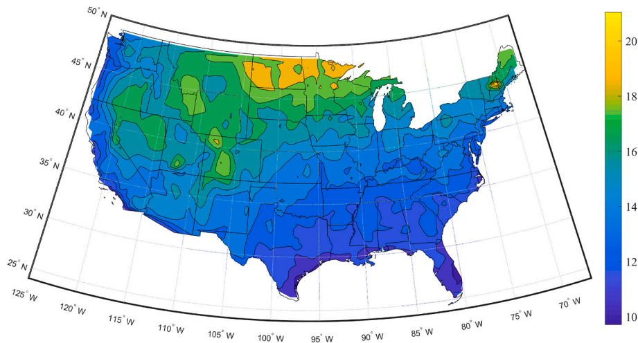
Fig. 13. \Delta\bar{T}_{TD} (°C) for a prescribed Climate Zone 7A “Medium Office” building across the U.S.
