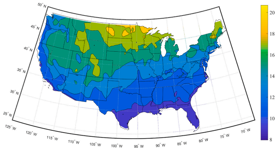
Fig. 19. \Delta \bar{T}_{TD} (°C) for a prescribed Climate Zone 4A "Large Hotel" building across the U.S.
