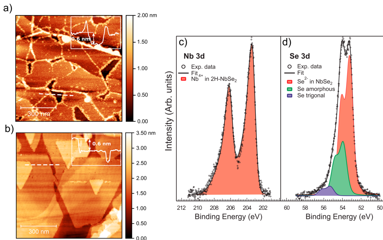
Figure 2. Morphological and spectroscopic characterization of NbSe 2 thin films grown by molecular beam epitaxy. (a,b) AFM images of NbSe 2 grown on BLG/SiC and on HOPG, respectively. The insets show height profiles along the white lines in (a,b). (c) Fitted Nb 3d and (d) Se 3d core level XPS spectra of NbSe 2 /BLG/SiC. The Se 3d core level spectrum in Figure 2d can be deconvoluted into three components with the main component corresponding to Se 2- in NbSe 2 (Se 3d 5/2 peak at 53.25 eV, red component). The two minor components can be ascribed to residual amorphous Se (green component at 53.95 eV) and trigonal Se (blue component at 55.35 eV).
