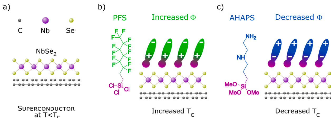
Figure 1. Schematic representation of our approach to manipulate the critical temperature T_C of NbSe 2 . (a) Large-area NbSe 2 monolayer grown on epitaxial bilayer graphene (NbSe 2 /BLG/SiC); molecular functionalization of the NbSe 2 monolayer with (b) trichloro(1H,1H,2H,2H-perfluorooctyl)silane (PFS) and (c) N-[3-(trimethoxysilyl)propyl]ethylenediamine (AHAPS). The direction of the PFS (AHAPS) molecule's permanent dipole moment leads to an increase (decrease) of the work function ( \Phi ), which in turn causes an increase (decrease) of T_C , due to hole (electron) accumulation.
