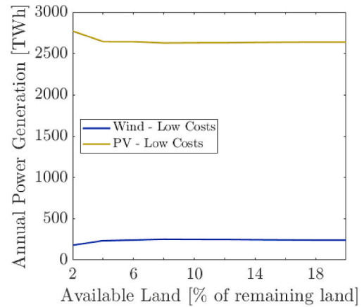
Fig. 6. Annual power generation from PV and wind power in MENA as a function of available land assuming low-costs for PV and batteries.
