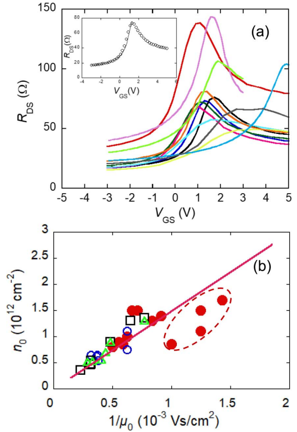
FIGURE 3. Different GFET channel transport properties across the silicon chip. (a) Drain resistance of the GFET's versus the gate voltage and inset shows the modelling results for the hole branch (line) of a GFET's. (b) Residual charge-carrier concentration versus inverse low-field mobility in the GFETs of gate lengths 0.5 \mu\text{m} (filled circles), 0.75 \mu\text{m} (open circles), 1 \mu\text{m} (squares), and 2 \mu\text{m} (triangles), located at different positions on the Si chip. The line corresponds to the product n_0 \cdot \mu_0 = 1.5 \cdot 10^{15} \text{ V}^{-1} \text{ s}^{-1} [14], [21], [25].
