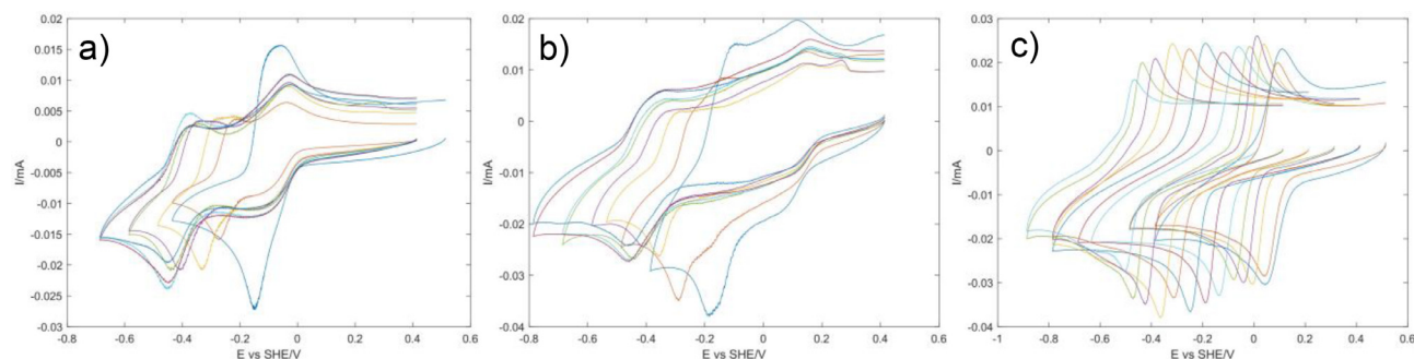
Fig. 11. Variation of CVs with pH for 1 mM a) 2H-NDI, pH 0–7, b) 2Br-NDI, pH 0–7 and c) 2DMA-NDI, pH 0–12. Sweep rate: 100 \text{ mV s}^{-1} . The pH increases to the left.
