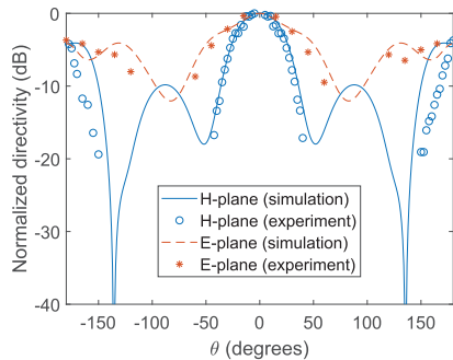
Fig. 4. Measured (symbols) and simulated (lines) H - and E -plane radiation patterns of one pixel in flat configuration.
