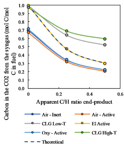
Figure 4. Carbon in the form of CO 2 in the syngas versus the apparent C/H ratio of the end product. The dashed line represents the theoretical amount of carbon in the form of CO 2 , according to reaction R1. The profiles shown in the graph for the air-inert and oxy-active cases are overlapping.
