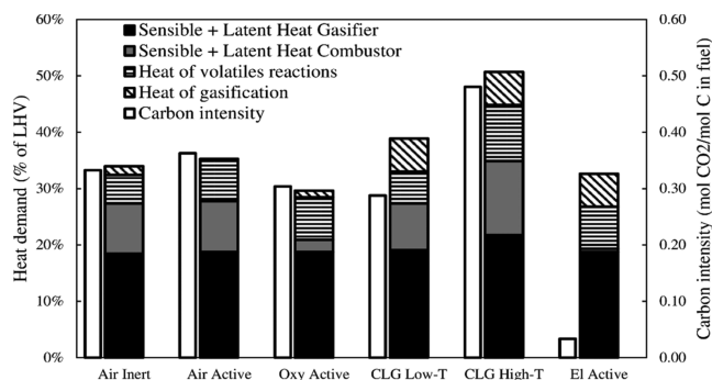
Figure 6. Contributions to the total heat demands of the various cases and the carbon intensities of the heat production methods. The latter represent the amounts of \text{CO}_2 produced in both the flue and raw gases due to the production of heat. The carbon intensity is represented by a white bar next to the stacked bars, and its values are displayed on the right vertical axis.
