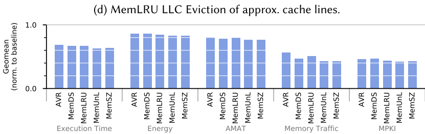
Fig. 11. Analysis of the compressor, error limiter, and LLC replacement policy introduced by MemSZ.
