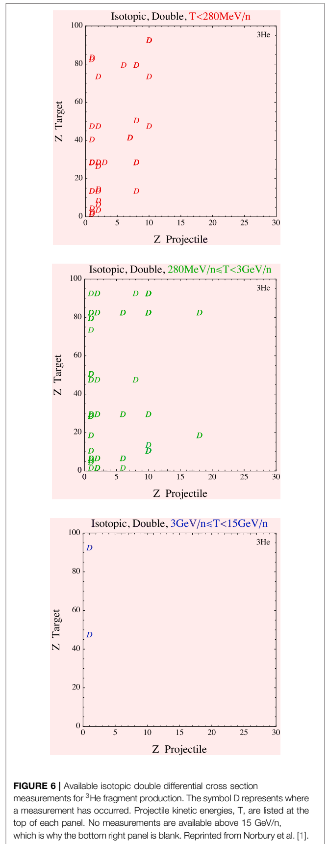
FIGURE 5 | Available isotopic double differential cross section measurements for {}^3\text{H} fragment production. The symbol D represents where a measurement has occurred. Projectile kinetic energies, T , are listed at the top of each panel. No measurements are available above 15 GeV/n, which is why the bottom right panel is blank. Reprinted from Norbury et al. [1].
