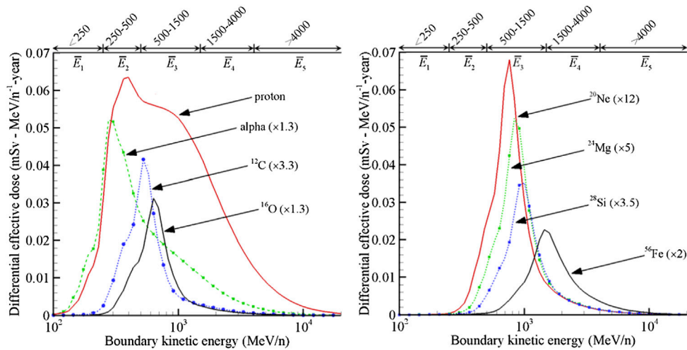
FIGURE 8 | Effective dose contributions as a function of external GCR energy behind 20 g/cm 2 of aluminum exposed to solar minimum GCR. Reprinted from Slaba and Blattnig [46].
