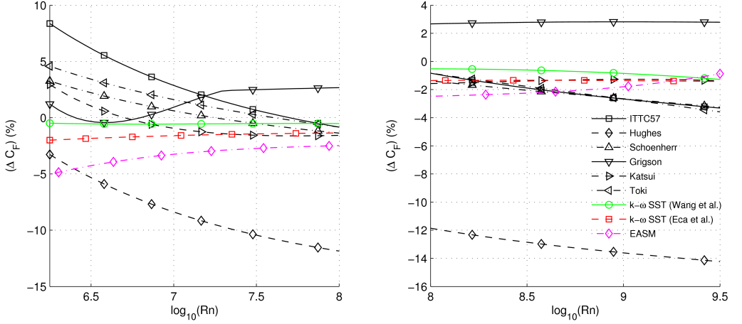
Figure 2.1: Friction lines in comparison to numerical friction line of SHIPFLOW with k - \omega SST turbulence model, from study conducted in Paper I
