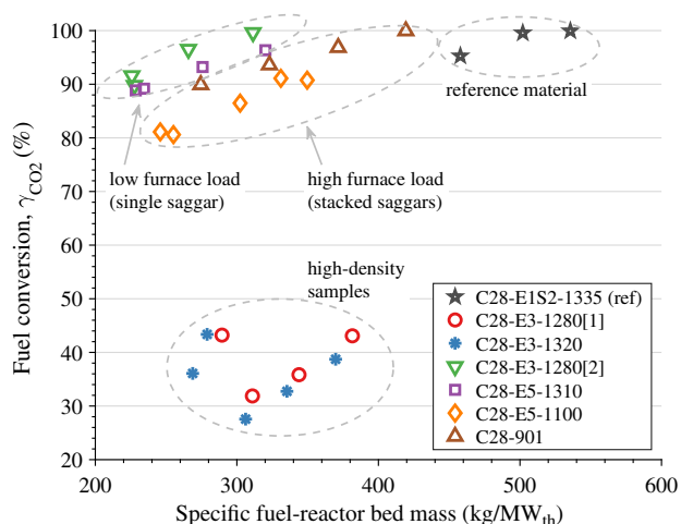
Figure 7. Fuel conversion, i.e., CO_2 yield \gamma_{CO_2} , at varied specific fuel-reactor bed mass at 900\text{ }^\circ\text{C} for experiments performed in the 300 W unit. Data are shown for materials during upscaling and for the material selected during raw material substitution (C28-E1S2) (cf. Table 1). C28-901 is the same batch of material that was used for testing in the 10 kW unit.
