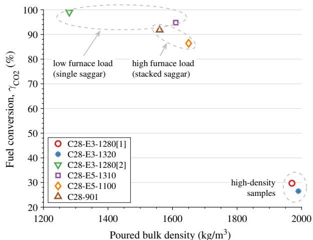
Figure 8. Oxygen-carrier reactivity expressed as fuel conversion, i.e., CO_2 yield \gamma_{CO_2} , at a fuel-reactor temperature of 900\text{ }^\circ\text{C} and a specific fuel-reactor bed mass of 300\text{ }kg\text{ }MW_{th}^{-1} (based on a data fit) as a function of poured bulk density (ISO 3923-1:2008). Data are shown for materials during upscaling. C28-901 is the same batch of material that was used for testing in the 10 kW unit.
