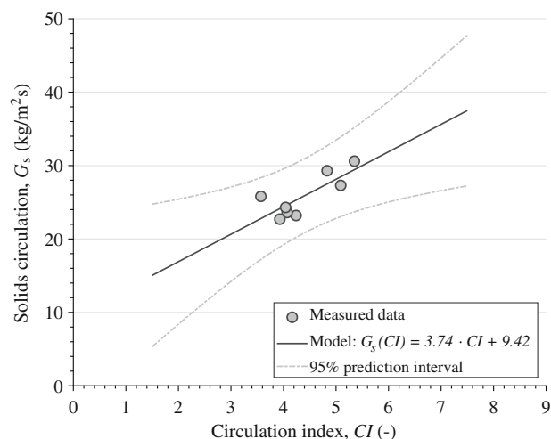
Figure 9. Correlation and modelling of solids circulation, G_s , as a function of the circulation index, CI , measured for oxygen-carrier material C28-901 in the 10 kW unit. Solids circulation was measured by means of feeding small batches of solid fuel during hot operation.
