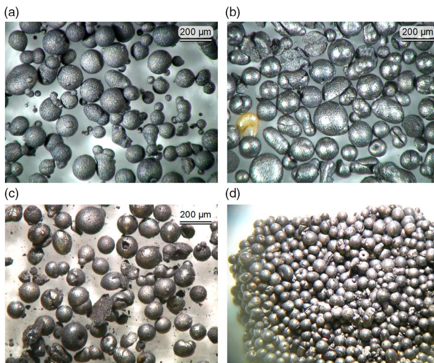
Figure 14. Light microscope images of different oxygen-carrier samples: a) fresh material, b) sample from AR after campaign, c) sample from FR after campaign, and d) agglomerate from FR after campaign. No scale is available for part (d), but particles are similar in size as those in parts (b) and (c). Differences in sheen between the subfigures are due to lighting.
