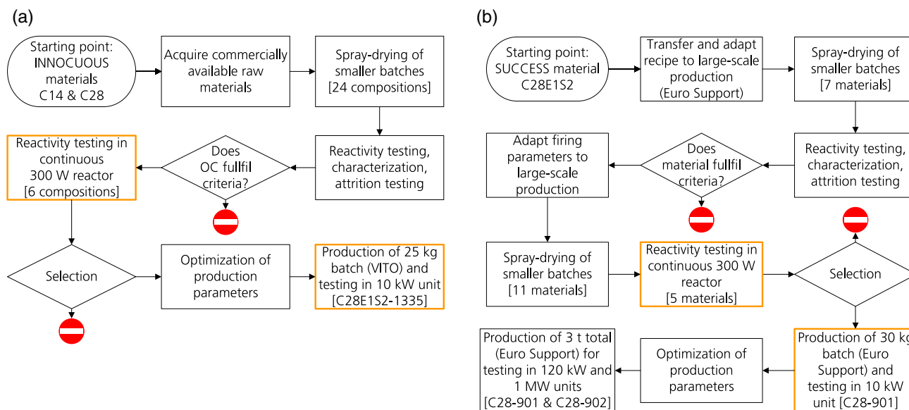
Figure 2. Detailed development schemes of calcium manganese-based oxygen carriers in the Success project for the tasks a) raw material substitution and b) upscaling.
