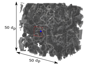
Spherical particle diffusing in an arbitrary pore.
