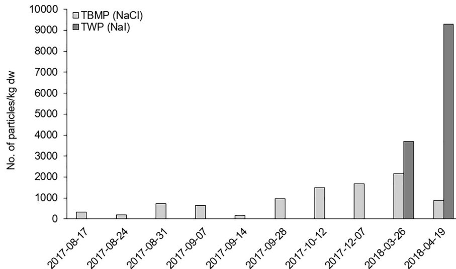
Fig. 9. TBMP and TWP \geq 100 \mu\text{m} in samples from sweepsand collected between 2017-08-17 and 2018-04-19. Light bars depict No. of particles/kg dw when separated with NaCl Dark bars depict No. of particles/kg dw when density separated with NaI.
