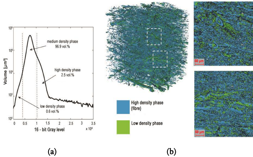
Figure 11: EAA-CNF-20 (a) X-ray microtomography data showing three density phases for the EAA-CNF-20 material, (b) 3D reconstruction of the (blue) high density fiber phase and of the (green) low density phase.
