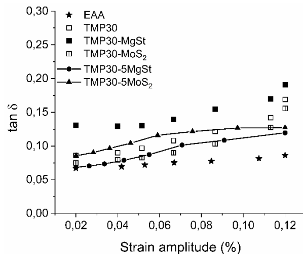
Figure 30: The mechanical loss factor as a function of applied strain amplitude for 30 wt% TMP samples containing different amounts of \text{MoS}_2 and \text{MgSt} .
