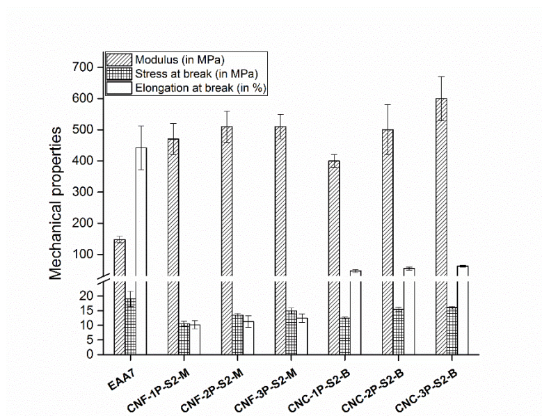
Figure 26: The mechanical properties of CNF- and CNC-reinforced samples compounded using the S2 screw design and shaped with the Maddock type barrier screw (CNF) and Maillefer barrier screw (CNC).
