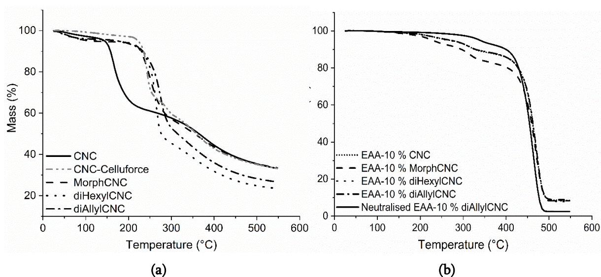
Figure 17: Thermogravimetric curves showing the thermal degradation of (a) unmodified CNC and azetidinium-grafted CNC before mixing with polymer and (b) of their compression-moulded composites.
