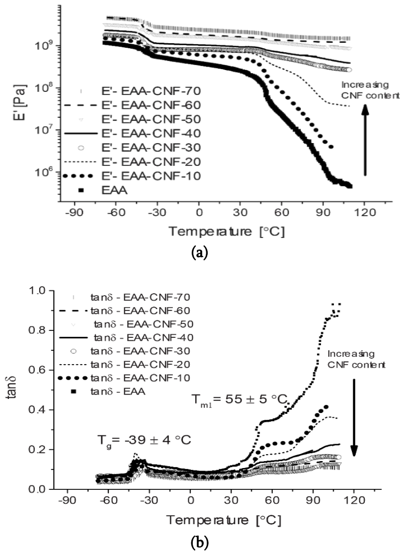
Figure 28: (a) Storage modulus ( E' ) and (b) loss factor ( \tan \delta ) of CNF-EAA composites measured at a constant strain amplitude at temperature from -80 to 110 °C.
