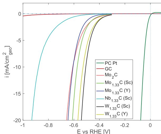
Figure 1. Hydrogen evolution reaction for different MXenes, with Pt and glassy carbon (GC) for comparison. Pt, to the far right is a near perfect catalyst for HER, while GC has virtually no activity. The parenthesis in the legend entries indicates whether the MXene was exfoliated from a Sc or Y based MAX phase.
