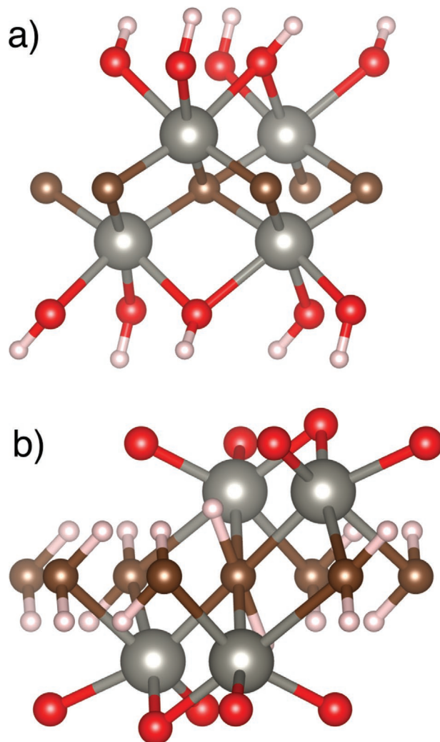
Figure 6. Illustration showing the atomic structure of W 1.33 CO 2 , a) for H atoms adsorbed to O on the surface, and b) to the C in the vacancy. In a) each O bonds with 1 H and in b) each C bonds with two H. Brown, gray, red, and white spheres correspond to C, W, O, and H, respectively.
