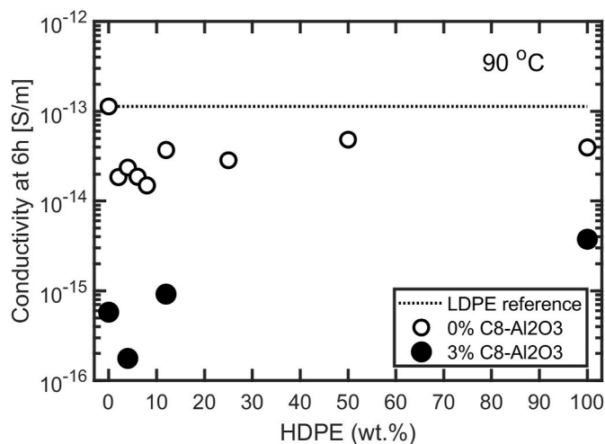
Fig. 8. Electrical conductivity (6h, 90 °C, 32 kV/mm) as a function of HDPE wt. %, for LDPE blends with and without 3 wt% C 8 -Al 2 O 3 in the LDPE.
