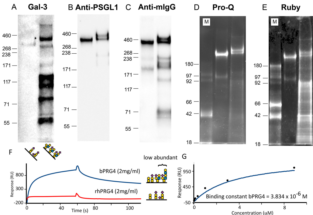
Figure 4. Galectin-3 binding to core 2 glycans. To display the difference of galectin-3 binding between core 1 and core 2, 1 \mu\text{g} of PSGL-1/mlgG2b (with core 1 glycans) (lane 1) and PSGL-1/mlgG2b + GCNT1 transferase (with core 2 glycans) (lane 2), immunoprecipitated from CHO tissue culture, were loaded, separated, blotted, and subsequently stained with biotinylated galectin-3 (panel A). Below the lanes, representative oligosaccharide cartoons show dominant O-glycans found on the two PSGL-1/mlgG2b glycoforms as described elsewhere. PSGL-1/mlgG2b monomers were detected in the area between 268–460 kDa, showing intense staining of the PSGL-1/mlgG2b expressed in CHO cells transfected with the GCNT1 transferase but less staining with the PSGL-1/mlgG2b with core 1 glycans. The same samples (50 ng each) were also separated, blotted, and stained by anti-PSGL1 (panel B) and anti-mouse IgG (mIgG) (panel C) antibodies in separate experiments, confirming similar concentration of the two constructs. The figure represents a typical result performed under optimized conditions from a selection of three repeats. For control, samples (1 \mu\text{g} each) loaded in the same order were separated and gels were stained for sugars using Pro-Q Emerald (panel D) and for proteins using Ruby (panel E). The gels include a molecular weight marker lane (M) identifying the PSGL-1/mlgG2b proteins with a molecular mass >180 kDa. F, SPR experiment showing binding of bovine lubricin (bPRG4) to recombinant galectin-3, whereas rhPRG4 did not bind. Inserted are cartoons showing prominent O-glycans on the two proteins, with symbol key displayed in Fig. 1A. G, calculation of binding constant of bPRG4/galectin-3 from SPR based on molecular mass of bPRG4 estimated to 220 kDa.
