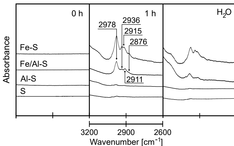
Figure 5.5: Background subtracted IR spectra recorded at 250 °C in Ar after exposing S, Al-S, Fe-S and Fe/Al-S in the H + -form to 2% CH 4 /Ar at 250 °C for 0 and 1 hours and to 4% H 2 O/Ar at 250 °C for 30 minutes. The background spectra were taken in Ar at 250 °C after the pretreatment in 500 ppm N 2 O/Ar and before CH 4 exposure.
