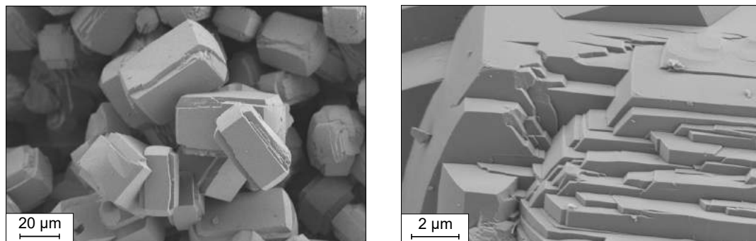
Figure 4.1: SEM images of the zeotype crystallites in the as synthesized form (left column) and H^+ -form (right column), and TEM image of the 10 MR of a portion of pure silicalite crystallite, together with schematic representation of the 10 MR.
