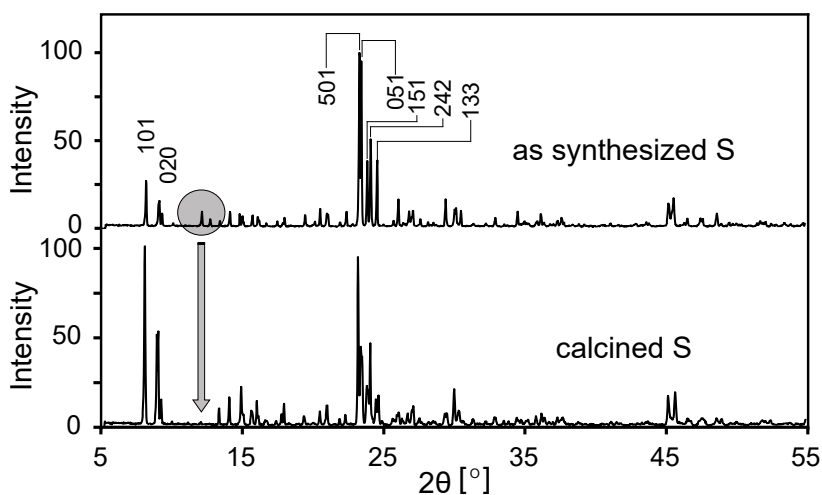
Figure 4.4: X-ray diffractograms of S before and after calcination, together with the Miller indices of the crystal planes associated to the diffraction peaks with the highest intensities. The disappearance of the peaks associated to the SDA after calcination is shown by the grey circle and arrow.
