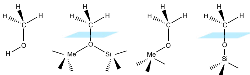
Figure 5.1: Schematic representation of the methanol molecule and methoxy groups adsorbed on BASs (Me = metal), other metal sites and terminal silanol groups (from left to right). The presence and the absence of the blue mirrors indicate the C_{3v} and the C_s type of symmetries, respectively, of the -\text{CH}_3 groups.
