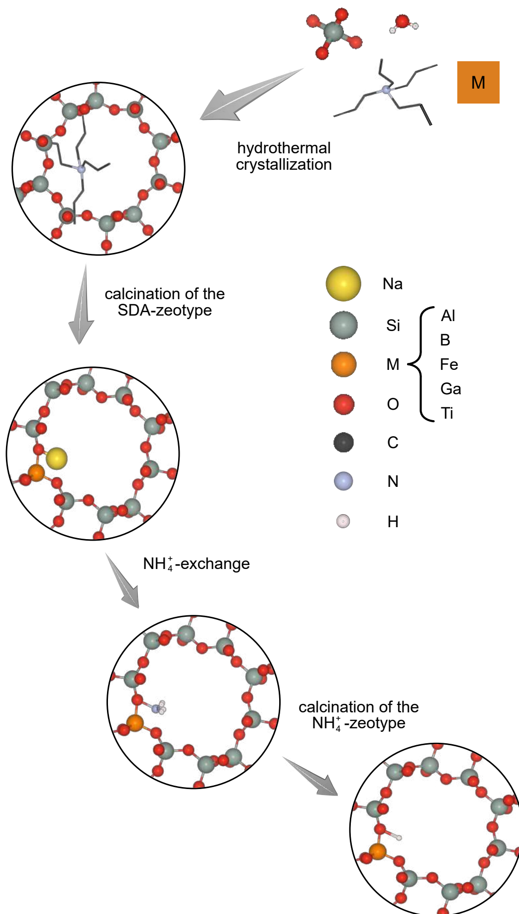
Figure 2.5: Schematic representation of the synthesis steps from the sol-gel preparation to the formation of the zeotype samples in the final form. Drawing produced by Vesta.[13]
