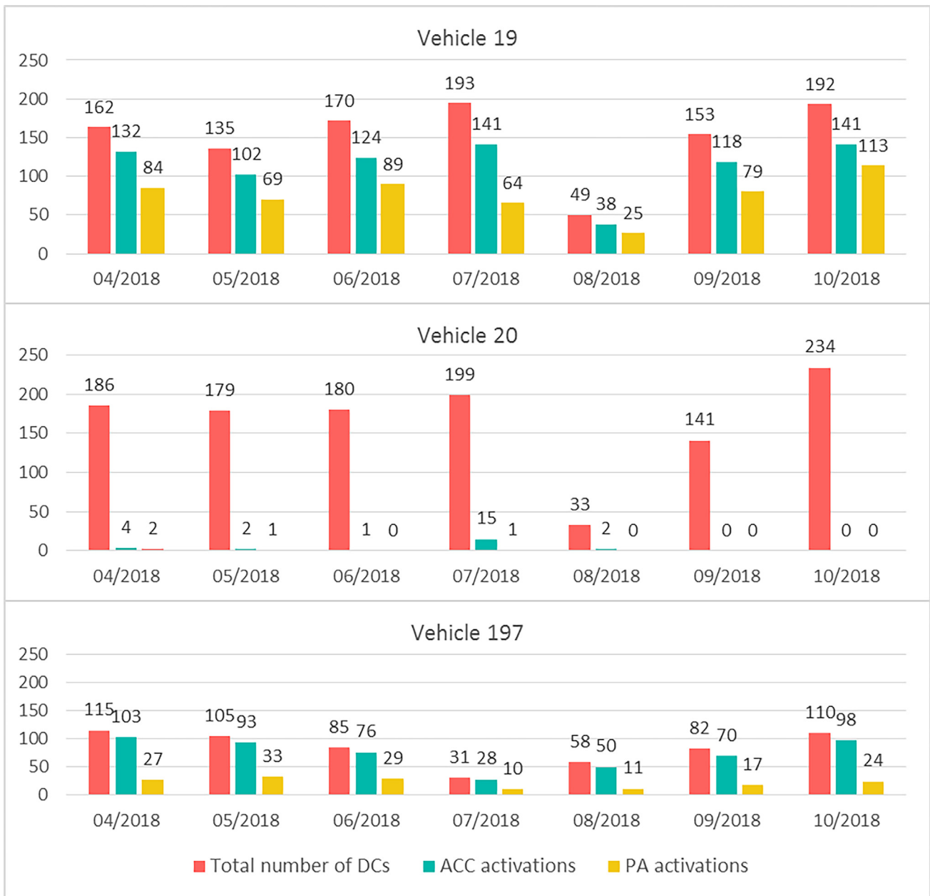
Fig. 3. Different use levels regarding ACC and PA for drivers of vehicles 19, 20 and 197.
