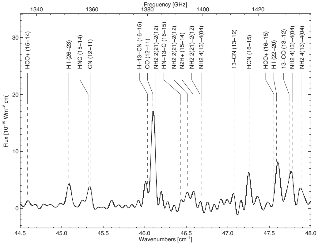
Figure A11. SPIRE spectrum 44.5–48.0 cm -1 .
