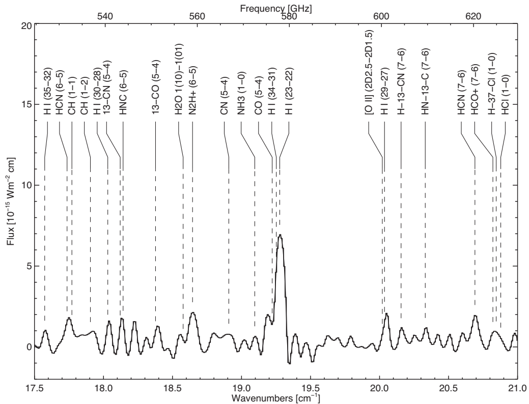
Figure A2. SPIRE spectrum 17.5–21.0 cm -1 .
