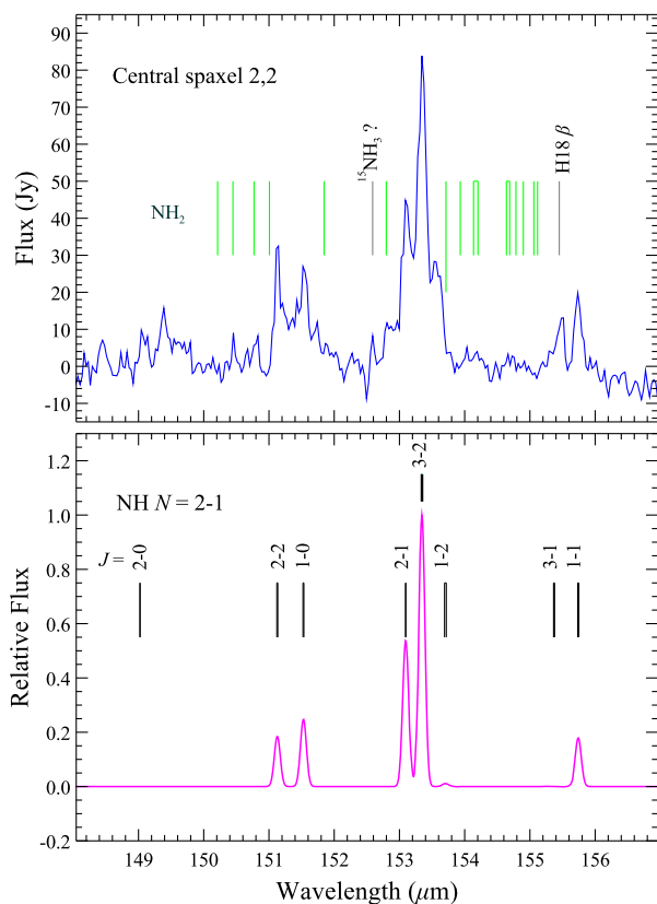
Figure 8. NH N = 2-1 complex between 151 and 156 \mu\text{m} . Top: Continuum-subtracted spectrum centred on \eta Car with vacuum wavelengths shown for H18 \beta , a weak, low significance identification of ^{15}\text{NH}_3 , and \text{NH}_2 transitions all with upper level energies below 1000 K. The spatial extent of NH coincides with the Homunculus lobes and skirt as demonstrated in Fig. 9. Bottom: A reference non-LTE model of NH over the full range of spin-rotation-hyperfine components, computed at 100 K and zero LSR velocity, convolved with the PACS resolution of 0.05 \mu\text{m} at 150 \mu\text{m} . The width of fiducial lines at each J state indicates the range of hyperfine transitions. Note that three of the eight spin rotation components contribute practically no measurable emission, consistent with their low transition probabilities.
