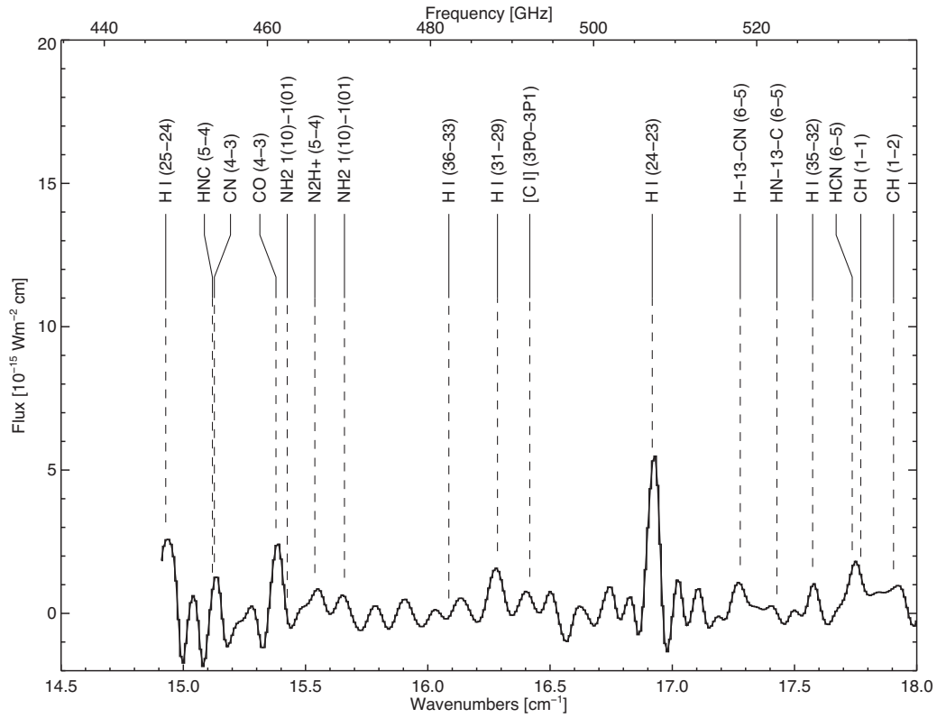
Figure A1. SPIRE spectrum 14.5–18.0 cm -1 . As commented in Section 2.2, the S/N exceeds 100 over most of the spectrum depicted in Figs A1 through A13. Most of the features in these spectra are real and promise to reveal even more line identifications. Note that, for all of the following spectral plots, the strong continuum has been subtracted to provide an optimized baseline for line identification.
