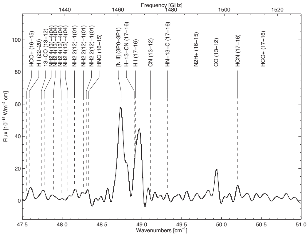
Figure A12. SPIRE spectrum 47.5–51.0 cm -1 .
