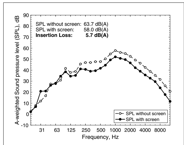
Figure 8. Measured L_{AFmax} spectra with and without screen at point P2, averaged over the two heights 1.2 and 1.5 m. A-weighted total insertion loss is 5.7 dB.
