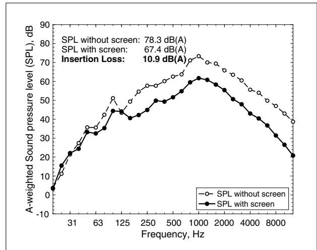
Figure 7. Measured L_{AFmax} spectra with and without screen at point P1, averaged over the two heights 1.2 and 1.5 m. A-weighted total insertion loss is 10.9 dB.
