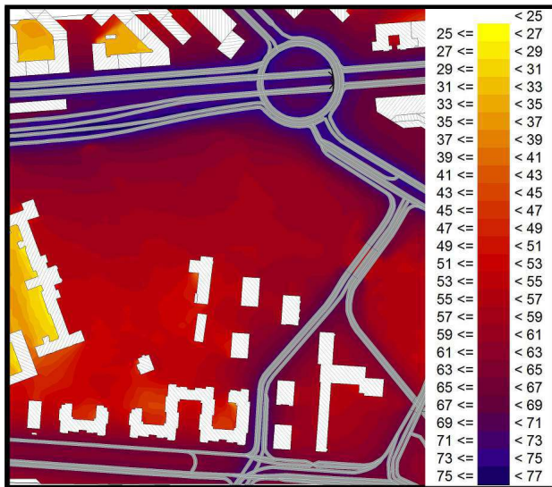
Figure 5. Predicted 24-hour equivalent noise level, L_{Aeq24h} (dB), at height 1.2 m.
