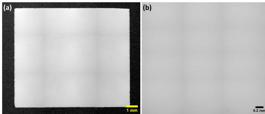
Figure A3. The optical micrographs of the as-built MAD542 processed by #3 printing parameters (laser power: 100 w; scan speed: 1300 mm/s; hatching distance: 50 μm; layer thickness: 20 μm). (a) The overview of the as-built cube and (b) the enlarged view with higher magnification (sample preparation: metallographic polishing).
