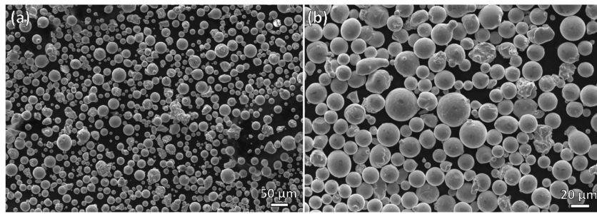
Figure A2. Secondary electron SEM micrographs of the virgin powders of the MAD542 superalloy for laser powder bed fusion. (a) at low magnification with an overall view and (b) at high magnification with a detailed view.
