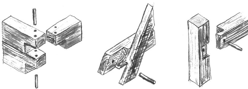
Figure 2.17: Nodal connections for a truss structure in wood inspired from timber trusses used in medieval church buildings as depicted in [104]. Sketch by the author.
