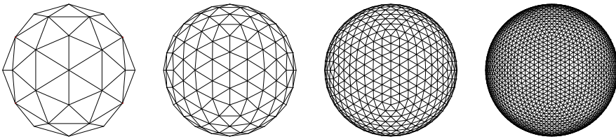
Figure 2.20: Illustrating increasing subdivision for a polygon approximation of a sphere.
