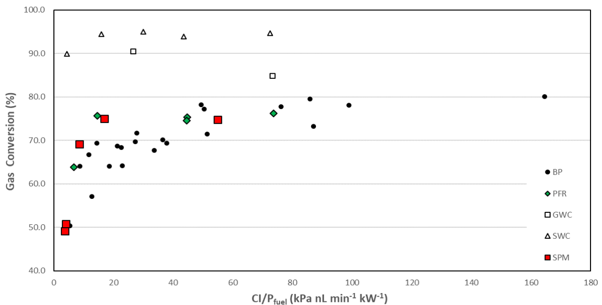
Figure 14 – Gas conversion efficiency vs. power-specific circulation index (Paper II)
