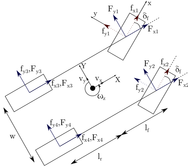
Figure 3.6: Two-track vehicle model.
