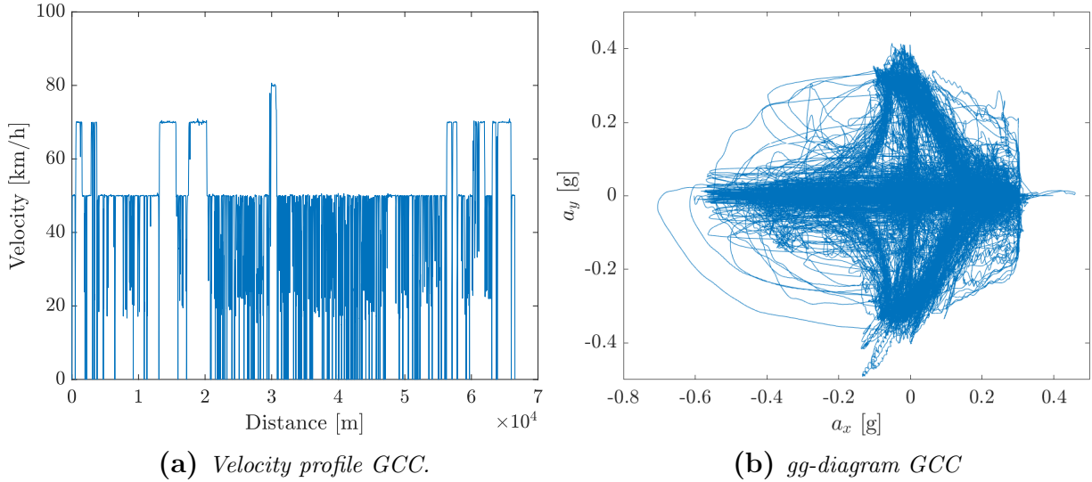
Figure 3.3: Driving pattern of Gothenburg City Cycle (GCC)
