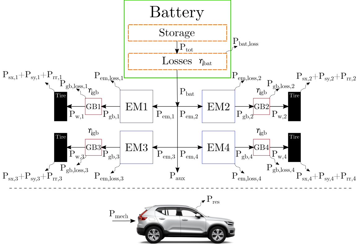
Figure 3.2: Power flow.
