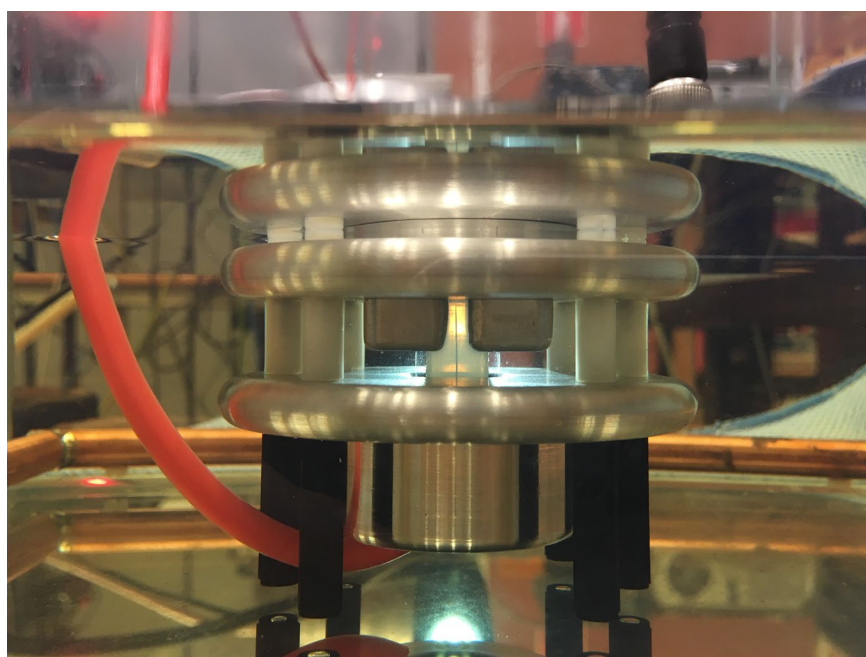
Figure 3.8: The submerged cell. The illumination shows the needle in the polymer. In the background the copper tubing which houses the heating elements is visible.
