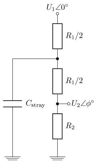
Figure 3.15. A model of the lumped parasitic capacitance.
