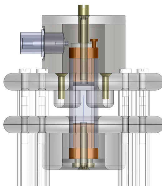
(b) The front of the cell, transparent view.
