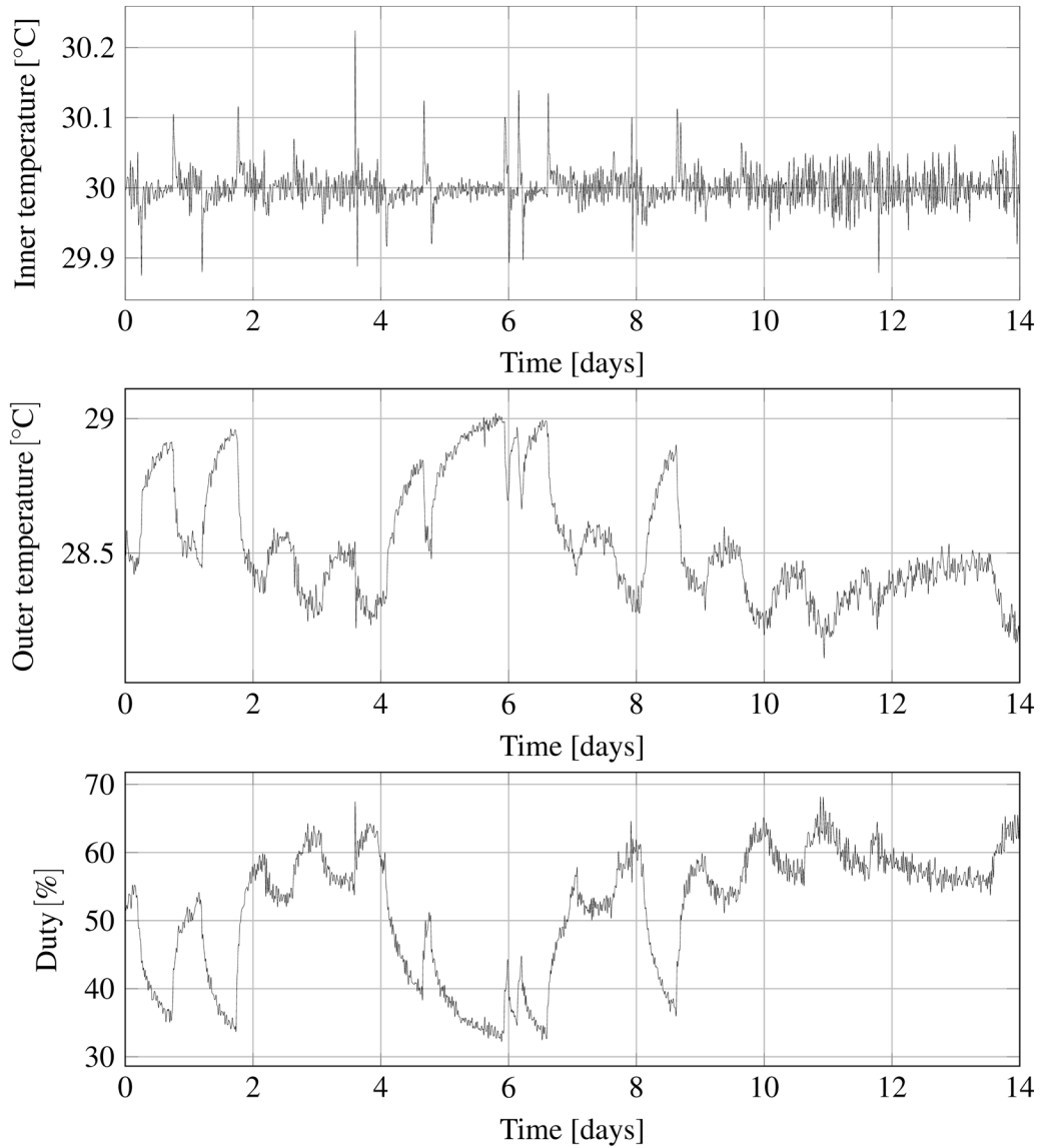
Figure 3.13 Temperature control of the reference impedance.
