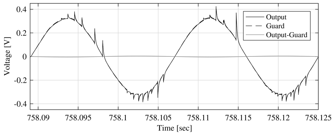
Figure 3.31: Guard performance.
