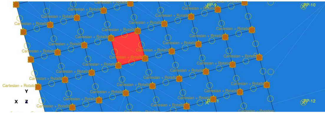
Figure 8 Partition of base slab and placement of springs at the partition's boundaries.
