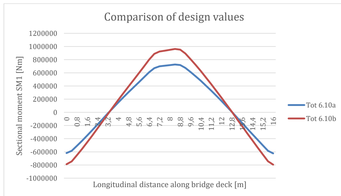
Figure 13. Comparison of design values of expressions 6.10a and 6.10b
