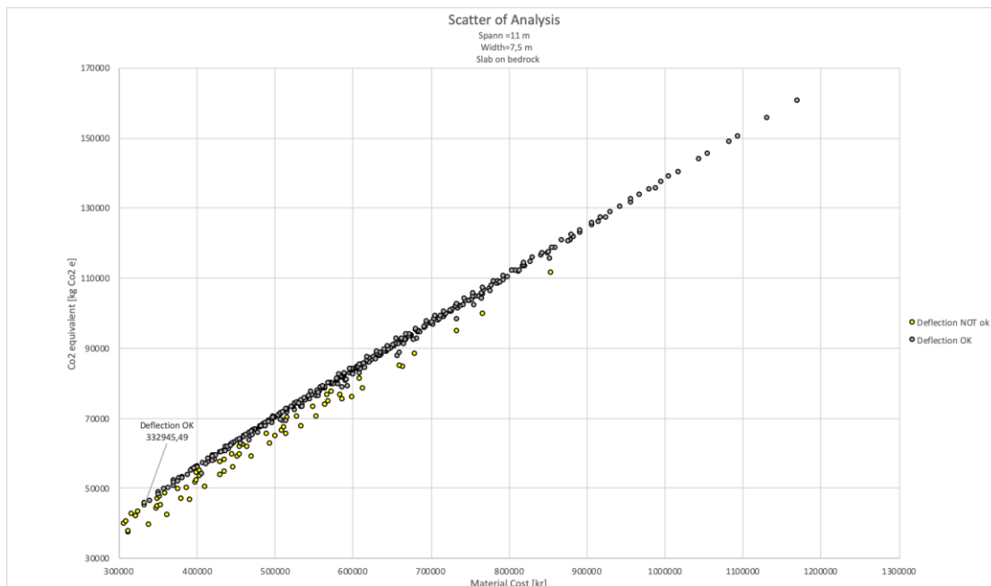
Figure 18 Set of 396 bridges. Same span length, width of bridge deck, height of frame legs and foundation conditions. Varying thickness of bridge deck, thickness of frame legs and skewed angle.
