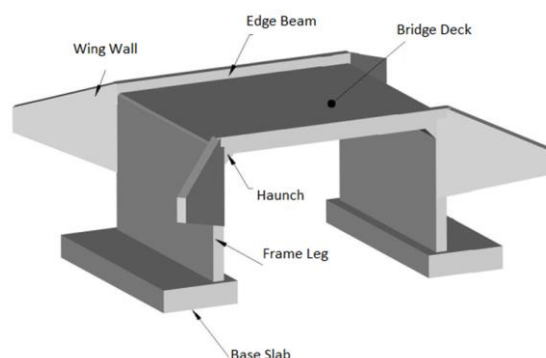
Figure 2 Different parts of a frame bridge (Vägverket, 1996)
