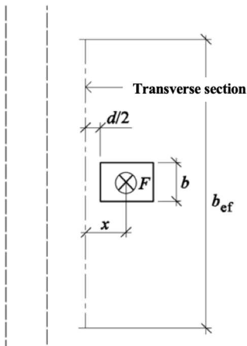
Figure 16 Effective width, b_{ef} , where shear force can be spread (Boverket, 2004)
