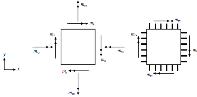
Figure 15 Definition of reinforcement moments. From (Engström, 2011)
