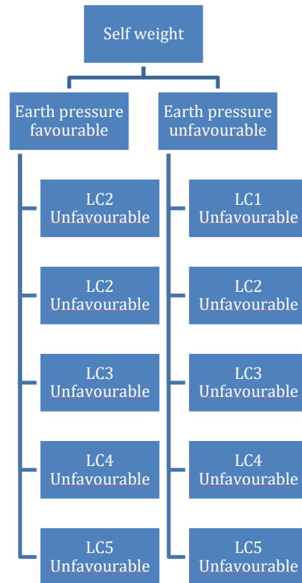
Figure 14 Final set of load combinations
