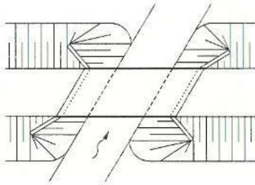
Figure 3 Frame bridge with skewed angle (Vägverket, 1996)
