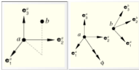
Figure 9 Cartesian connection translator type and rotational type
