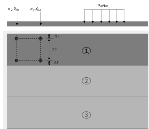
Figure 10 Application of Load Model 1 according to Eurocode
