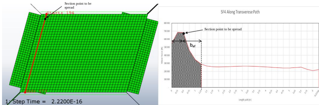
Figure 17. Spread of section point in model
