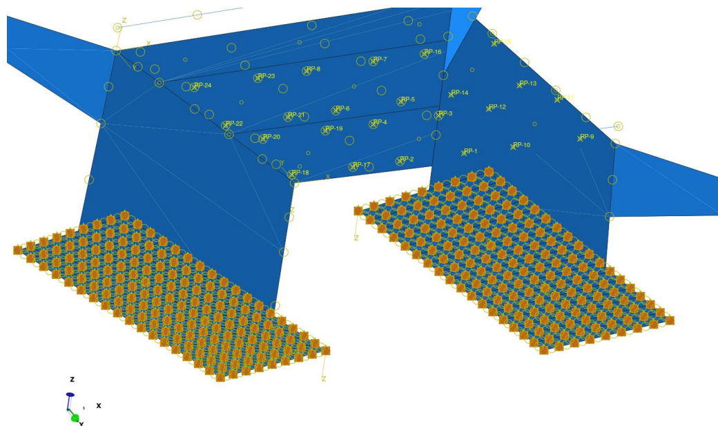
Figure 7 Spring connections between soil and base slab.
