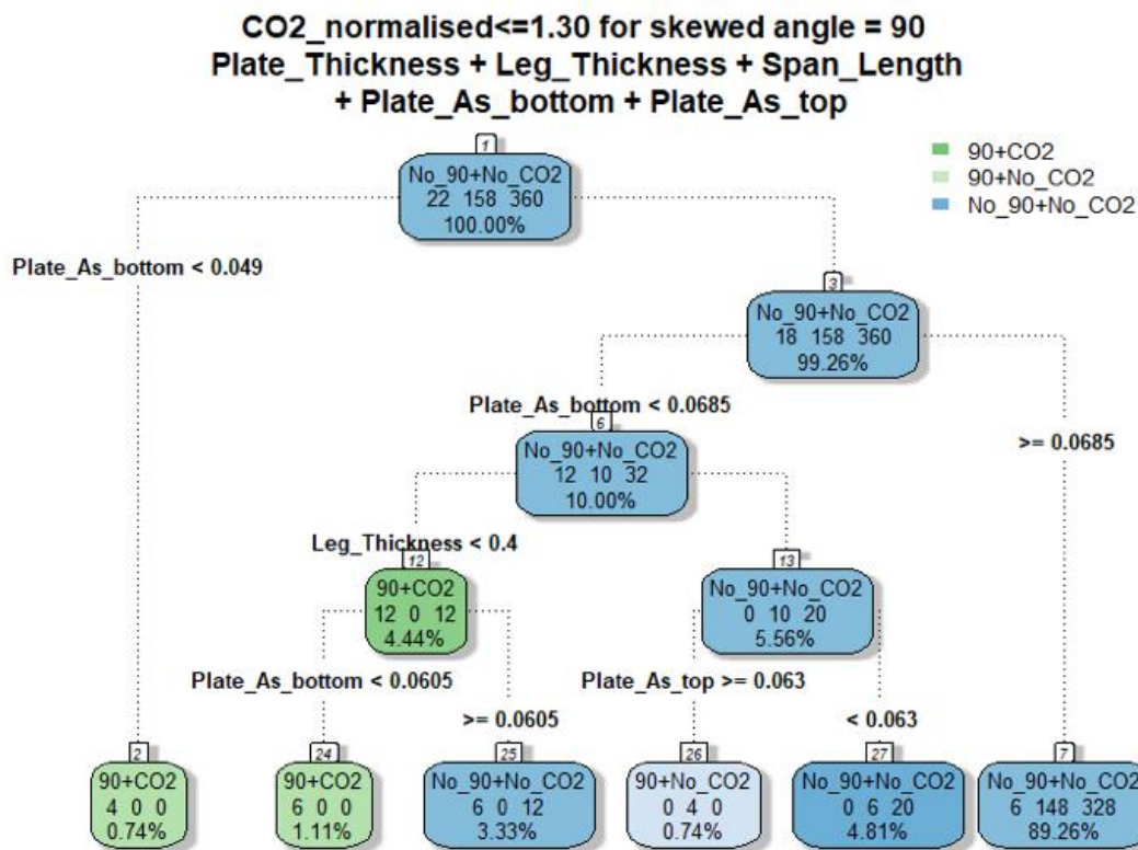
Figure 19 Decision tree from R with normalized CO 2 -equivalent less than 1.3 and skewed angle 90 degree. Every colored box are nodes and white box over every node is the numbering of the node.
