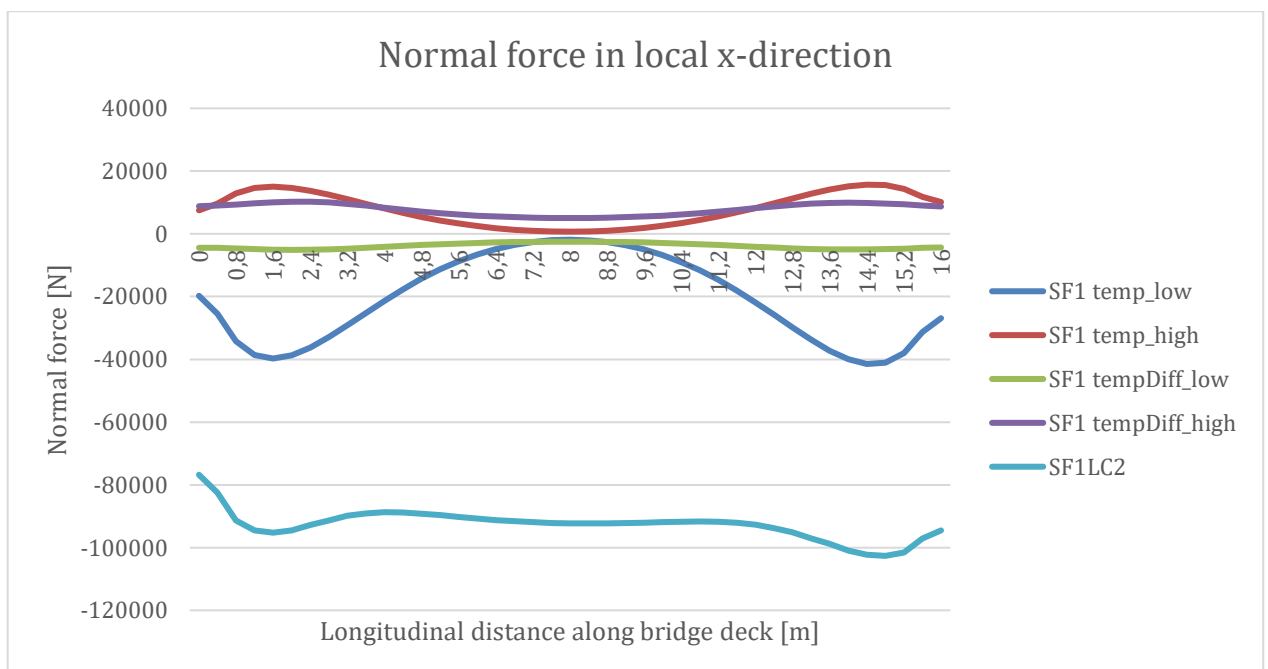
Figure 12, Normal force distribution along bridge deck
