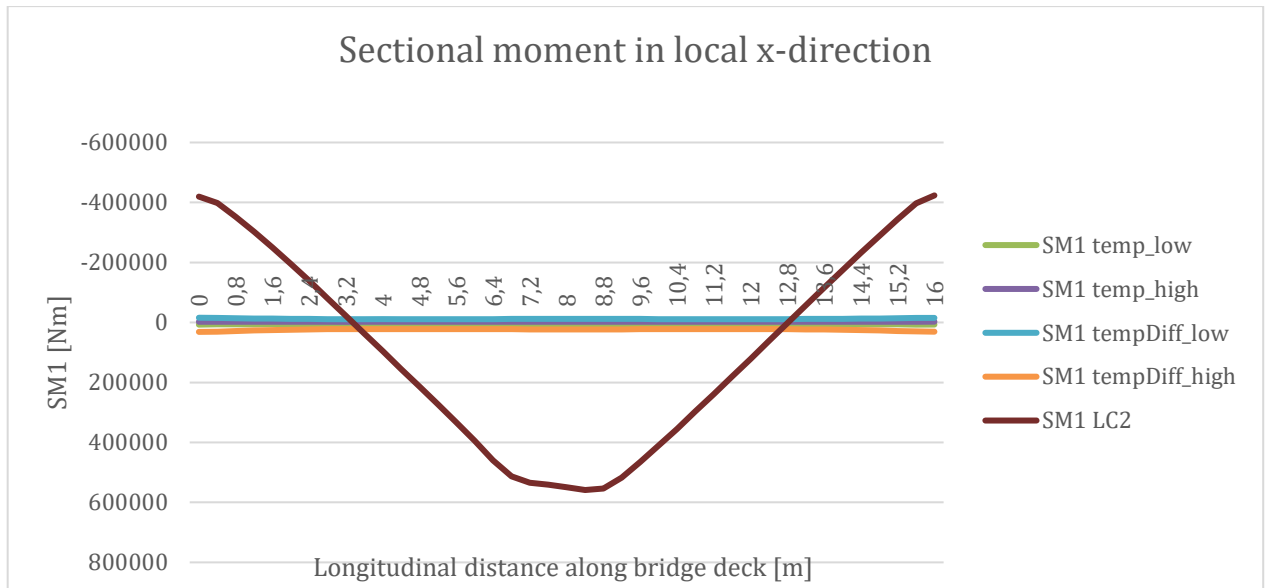
Figure 11, Sectional moment diagram in mid path of bridge deck
