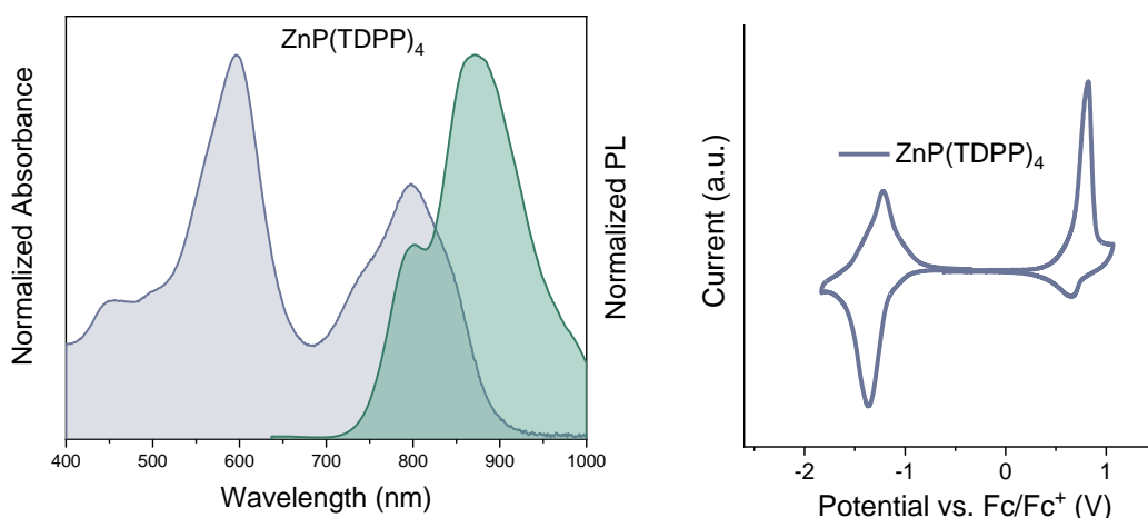
Figure 4.5. (a) Normalized Absorbance (purple) and PL (green) spectra of the \text{ZnP(TDPP)}_4 emitter in a toluene/pyridine 99:1 and concentration 10^{-6} M. (b) CV trace of \text{ZnP(TDPP)}_4 .
