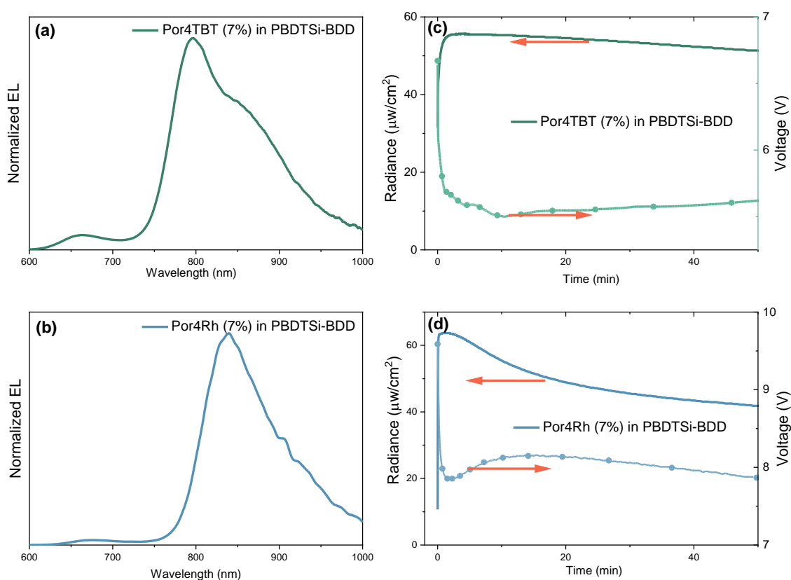
Figure 4.24. (a-b) Steady-state EL spectra for devices containing (a) Por4TBT and (b) Por4Rh in 7 mass% concentration. (c-d) Temporal evolution of the voltage and the radiance as a function of the guest selection, as identified in the legends.
