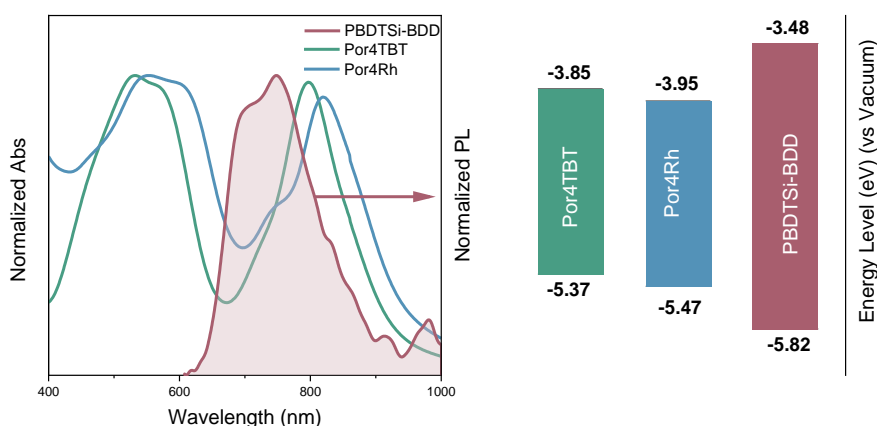
Figure 4.23. (a) Normalized absorption spectra of Por4TBT and Por4Rh and normalized PL spectrum of PBDTSi-BDD obtained in the solid state; (b) Energy level diagram of Por4TBT and polymer host PBDTSi-BDD used as the matrix in this study.
