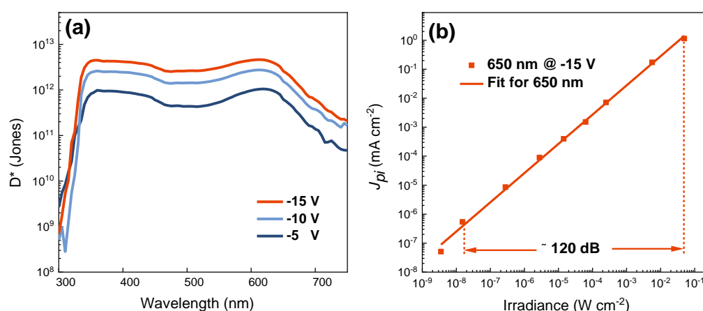
Figure 5.7. (a) Specific detectivity of the PM type OPDs at increasing reverse bias. (b) LDR of the PM type OPDs measured at -15 V bias under 650 nm light illumination, the solid red line is the linear fitting.
