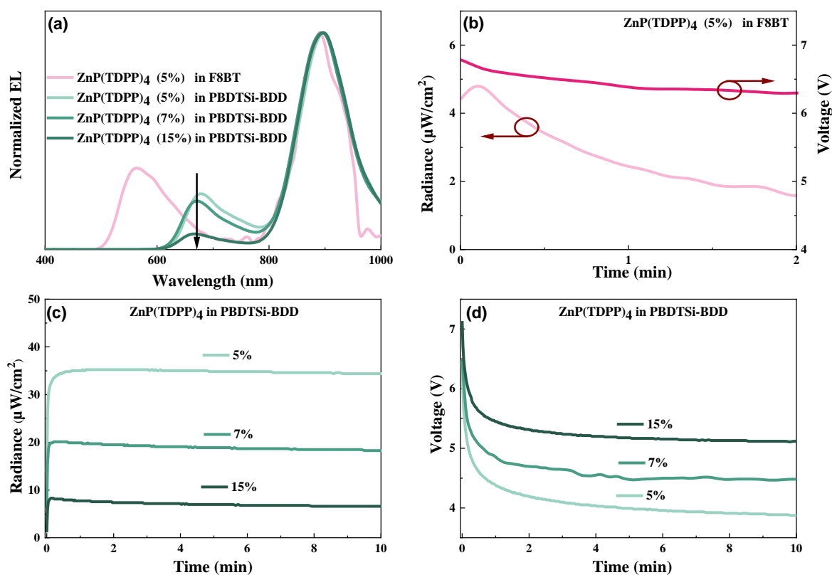
Figure 4.11 (a) Steady-state EL spectra as a function of host polymer with variable ZnP(TDPP) 4 concentrations. (b–d) Temporal evolution of the voltage and radiance as a function of host selection and ZnP(TDPP) 4 concentration, as identified in the legends.
