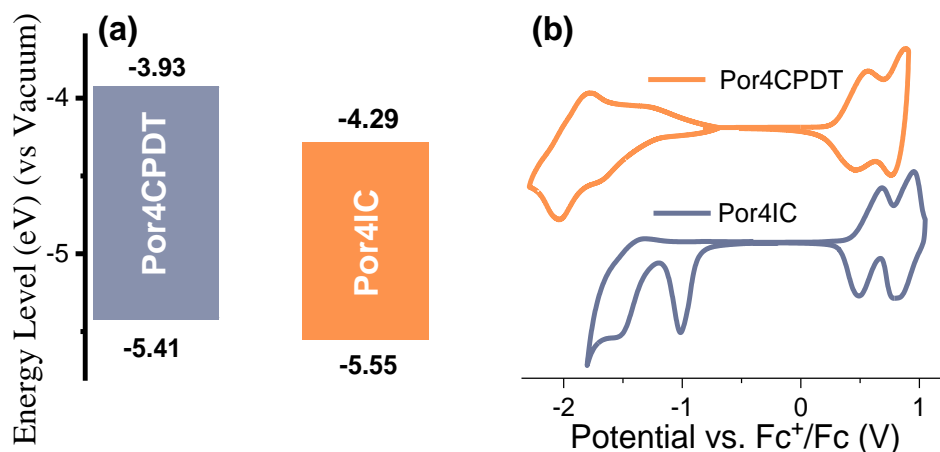
Figure 5.3. (a) Energy level diagram for Por4CPDT and Por4IC (b) the CV traces of Por4CPDT and Por4IC.
