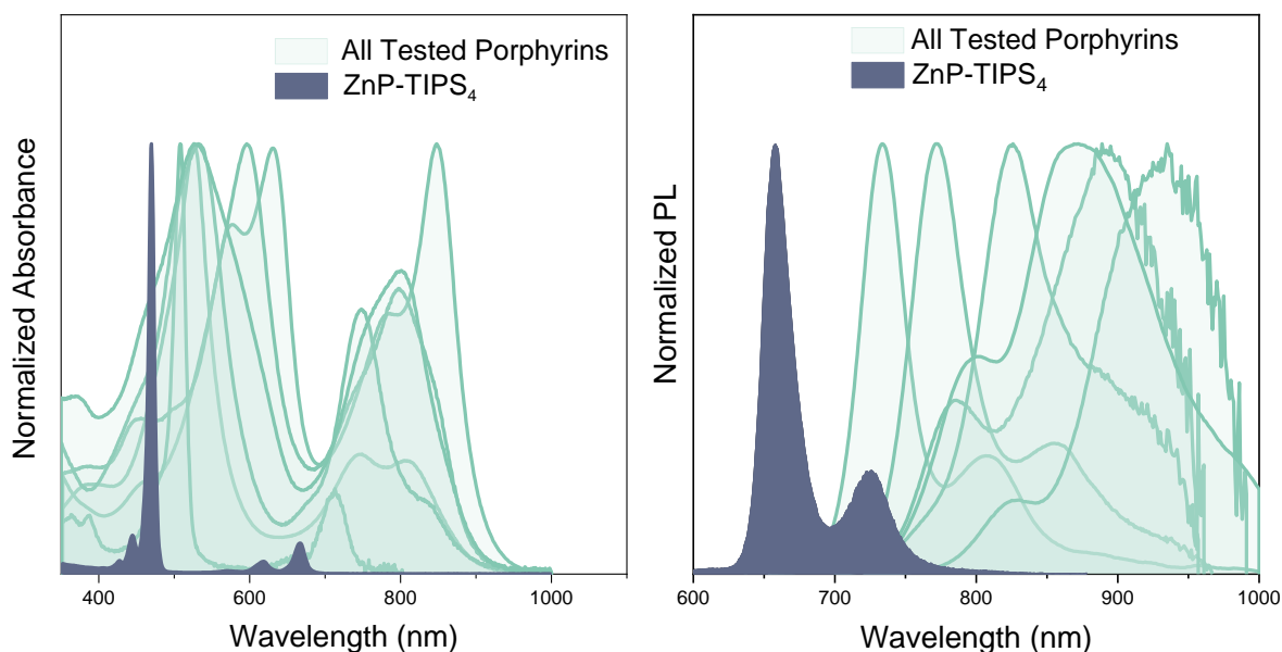
Figure 6.2. Normalized absorption (left) and PL (right) spectra of all porphyrins included in this thesis. The spectra belong to the solutions of the emitters while the concentration is 10^{-6} M. The purpose of the optical spectra in this Figure is to give an impression of the magnitude of the effect that the different strategies had in the spectra of the starting porphyrin core.
