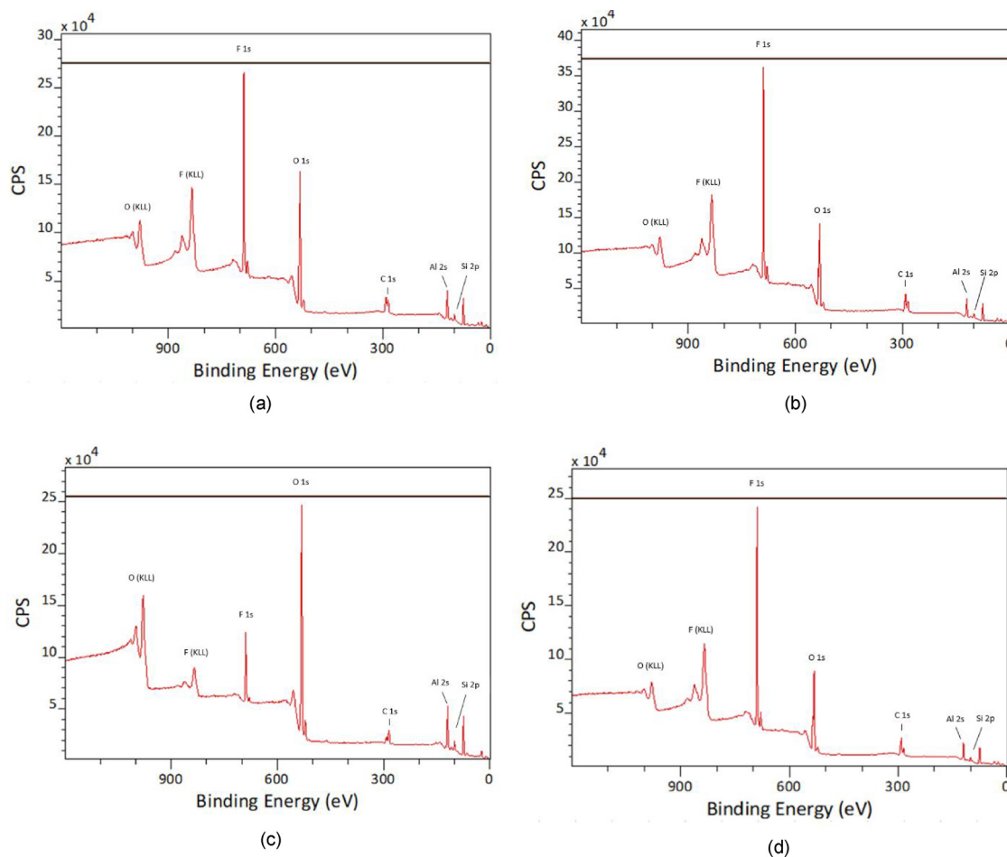
Fig. 6. XPS spectrums: (a) Reference Sample (b) Treated Sample (UV exposition 6 min) (c) Treated Sample (UV exposition 6 min + 30 min deionized water) (d) Sample Recovering (3 h at 165 °C).
