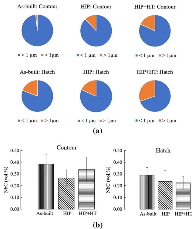
Fig. 9—(a) Pie charts showing the relative number of smaller (< 1 μm) and larger carbides (> 1 μm) in the contour and hatch regions of as-built, HIP and HIP + HT specimens. (b) Quantification of NbC content in the two regions for as-built, HIP and HIP + HT specimens.
