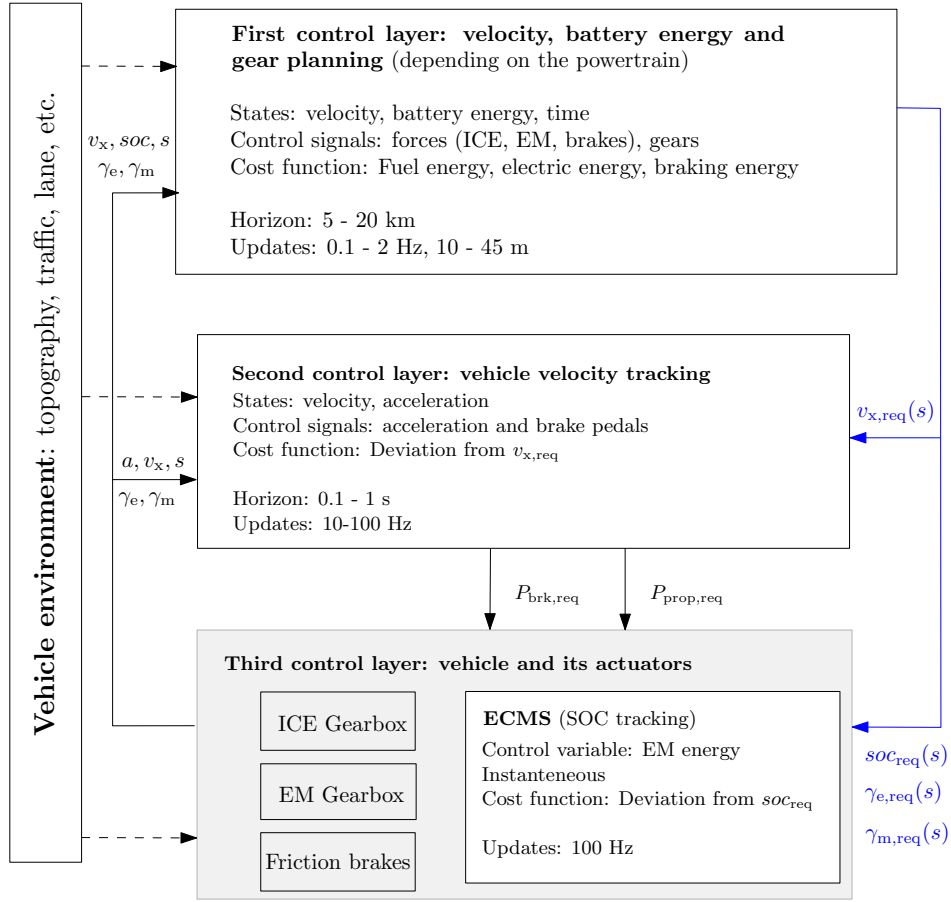
Figure 5.4: Overall control hierarchy, where v_{\text{req}} , \text{soc}_{\text{req}} , \gamma_{e,\text{req}} , and \gamma_{m,\text{req}} denote the optimal profile of the velocity, battery state of charge, ICE gear, and EM gear, respectively; P_{\text{prop,req}} and P_{\text{brk,req}} denote the propulsion and brake power requests; and signals a , v , s , \text{soc} , \gamma_e and \gamma_m are the feedback signals, where a denotes acceleration and s denotes the current distance traveled.
