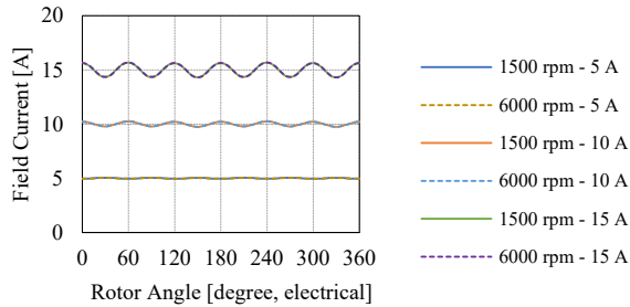
Fig. 17. Field current ripple due to airgap permeance variations at 1500 and 6000 rpm.
