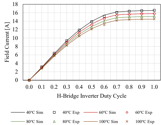
Fig. 5. Field current at 40, 60, 80 and 100°C.
