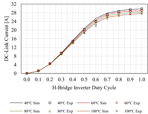
Fig. 6. DC-Link current at 40, 60, 80 and 100°C.
