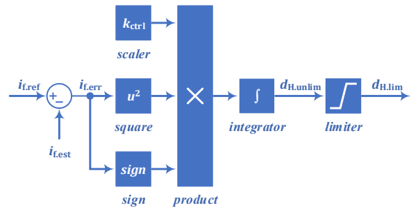
Fig. 14. Closed-loop field current control.
