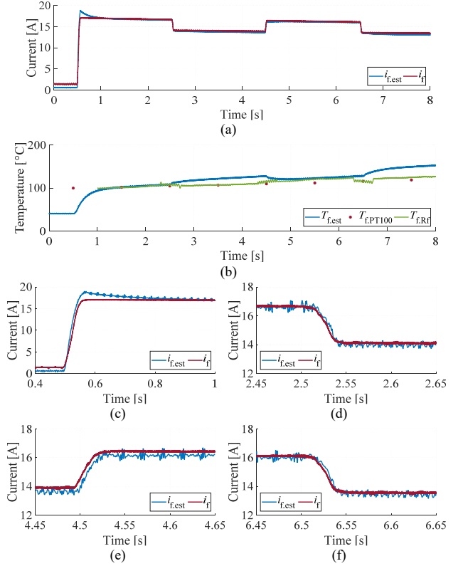
Fig. 13. Current and temperature tracking (experiment at 100°C). (a) field current from 0 to 8 s; (b) field winding temperature from 0 to 8 s; (c) field current from 0.40 to 1.00 s; (d) field current from 2.45 to 2.65 s; (e) field current from 4.45 to 4.65 s; (f) field current from 6.45 to 6.65 s.
