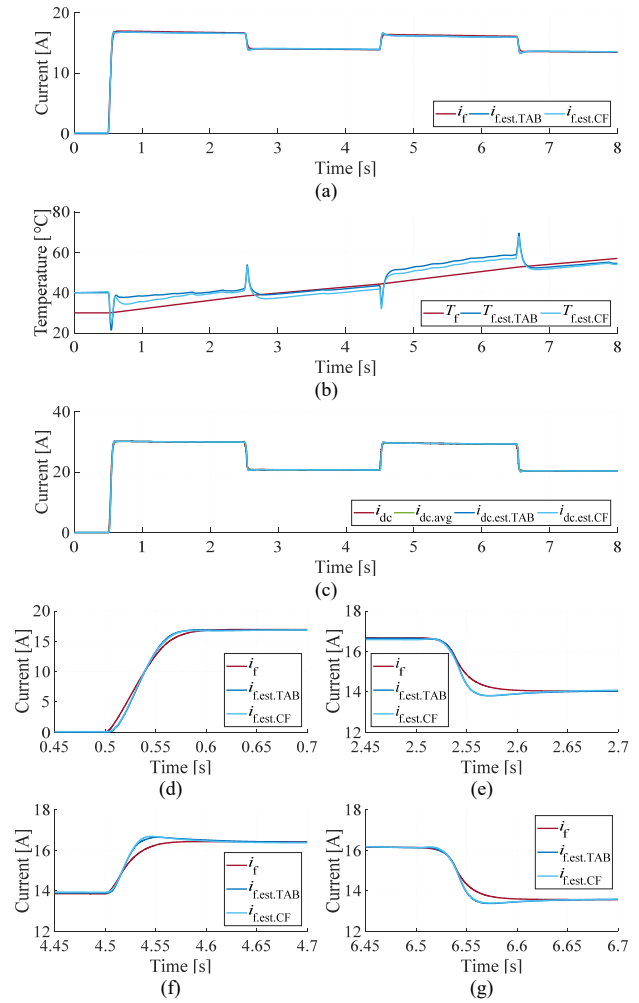
Fig. 11. Current and temperature tracking (simulation at 30^{\circ}\text{C} ).
