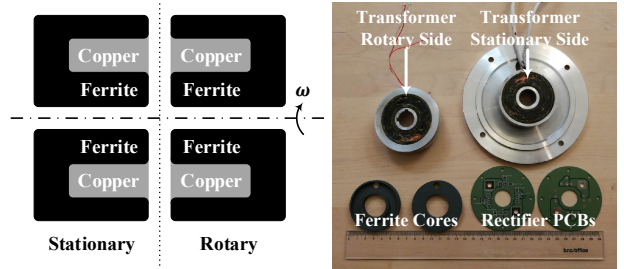
(a) topology with axial excitation (b) transformer, ferrite and rectifier Fig. 2. Rotary transformer.
