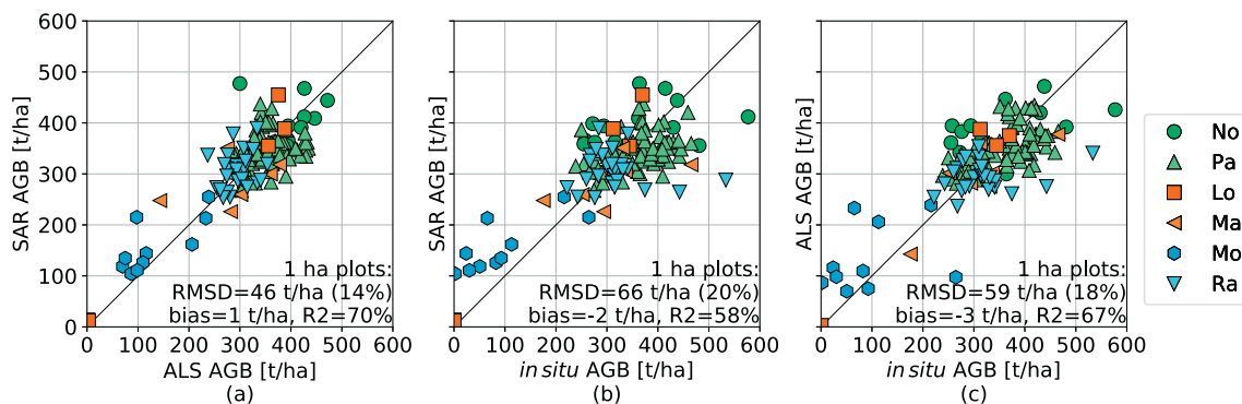
Fig. 9. Scatterplots showing pairwise comparisons of best-case single heading SAR-, ALS- and in situ -based AGB estimates for the 1 ha plots located within the six test sites, together with the associated performance metrics (bottom right corner). The SAR and ALS maps and in situ plots are shown in Figs. 6–7. AGB estimates were extracted from SAR and ALS maps by first averaging them to 100 m × 100 m and then linearly interpolating the AGB data to plot centres. Subplots show: (a) SAR AGB vs. ALS AGB, (b) SAR AGB vs. in situ AGB, and (c) ALS AGB vs. in situ AGB.
