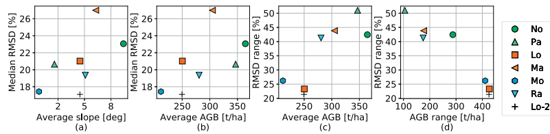
Fig. 10. Scatterplots of median RMSD against (a) average ground slope angle and (b) average AGB and relative RMSD range against (c) average AGB and (d) AGB range for all 6 test sites. The AGB statistics were calculated for estimation areas with AGB > 200 t/ha and the average test site properties were estimated at 2.25 ha scale.
