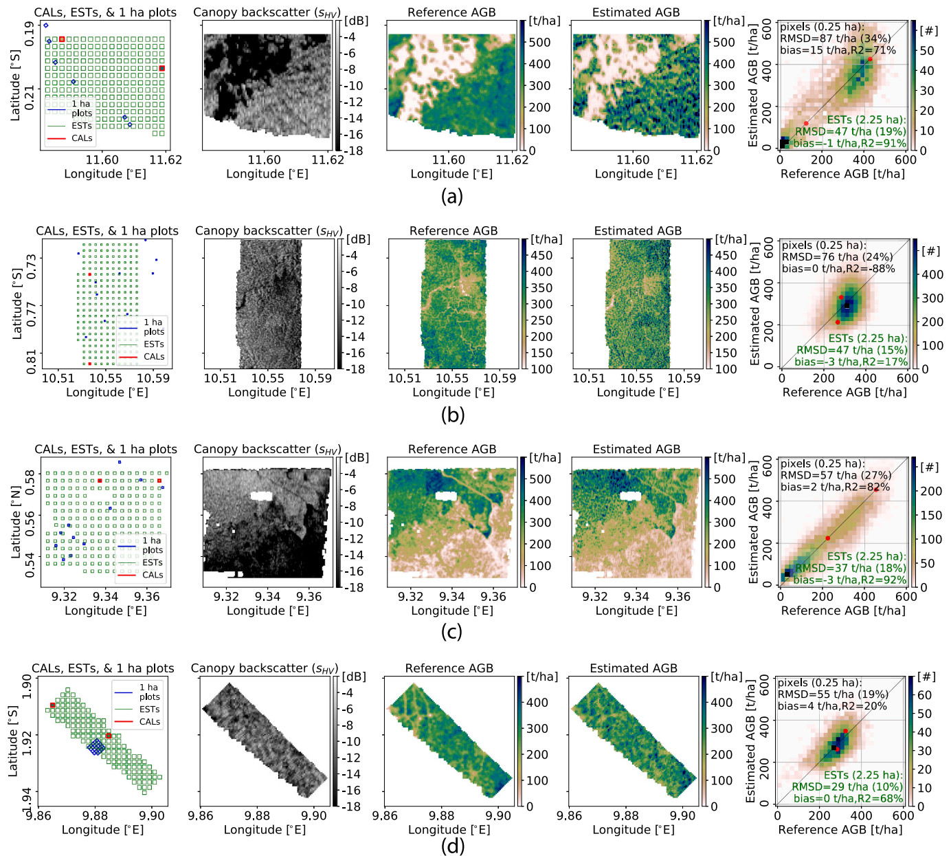
Fig. 7. Best-case AGB estimation results in (a) Lopé (heading: 275 deg), (b) Mabounié, (c) Mondah, and (d) Rabi, in Gabon. The leftmost plots show the 150 m \times 150 m estimation (EST) areas, two 150 m \times 150 m calibration (CAL) areas, and the 1 ha in situ plots. The next three plots show the canopy backscatter for HV polarisation ( s_{HV} ), the reference AGB map from ALS data, and the best-case AGB map estimated from SAR with CASINO. The rightmost plots show 2D histograms created using all pixels from the reference and estimated AGB maps, with the colour scale indicating the number of pixels; these plots include performance metrics for the 2.25 ha EST areas (bottom right corner) and the 0.25 ha pixels (top left corner). The red dots in the scatterplots show estimation results for the two CAL areas. The SAR data were acquired with the right-looking F-SAR system.
