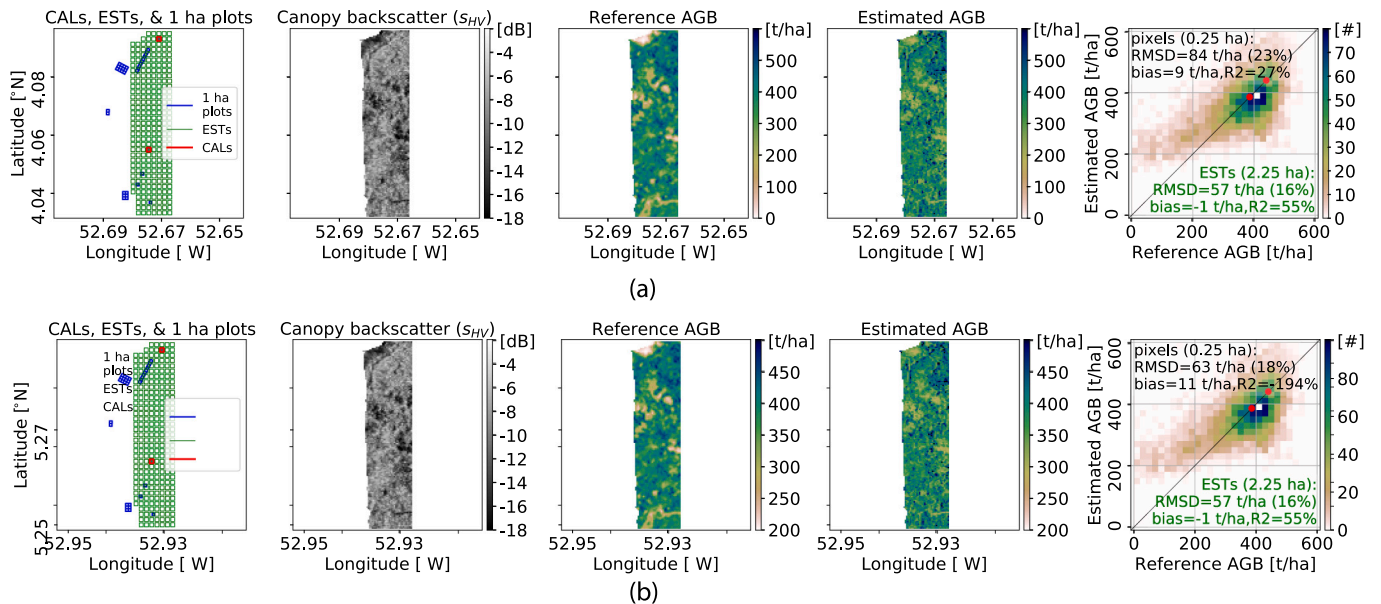
Fig. 6. Best-case AGB estimation results in (a) Nouragues and (b) Paracou, in French Guiana. The leftmost plots show the 150 m × 150 m estimation (EST) areas, two 150 m × 150 m calibration (CAL) areas, and the 1 ha in situ plots. The next three plots show the canopy backscatter for HV polarisation ( S_{HV} ), the reference AGB map from ALS data, and the best-case AGB map estimated from SAR with CASINO. The rightmost plots show 2D histograms created using all pixels from the reference and estimated AGB maps, with the colour scale indicating the number of pixels; these plots include performance metrics for the 2.25 ha EST areas (bottom right corner) and the 0.25 ha pixels (top left corner). The red dots in the scatterplots show estimation results for the two CAL areas. The SAR data were acquired with the left-looking SETHI system.
