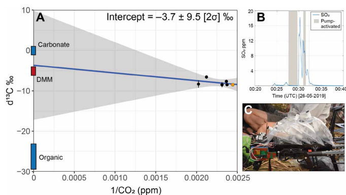
Fig. 6. Carbon isotope composition of Manam volcanic gas plume. (A) Isotopic composition and CO 2 concentration of samples collected by UAS in the plume emanating from the Southern Crater (black circles) and in clean ocean air (orange circle), extrapolated to 100% CO 2 by least squares linear regression (blue line). The gray shaded region shows the 95% confidence bounds on the regression. Uncertainties on the measurements are smaller than the symbol size unless shown. (B) The timing of bag sampling ("pump-activated") shown relative to SO 2 concentrations measured by co-located Multi-GAS instrument on 26 May 2019. Only the second pump activation was triggered within dense plume conditions (>5 ppm SO 2 ). (C) Sampling apparatus mounted on the multirotor UAS, comprising four Tedlar bags connected in series with the Multi-GAS and its pump. Image credit: T. Fischer.
