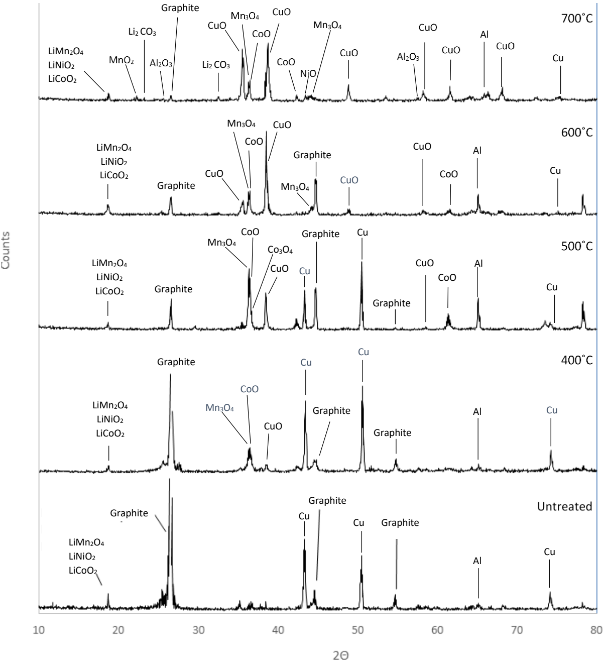
Figure 23: Comparison between the XRD spectrum of an untreated sample and the XRD spectra of the samples incinerated for 1.5 h at 400°C, 500°C, 600°C, and 700°C.
