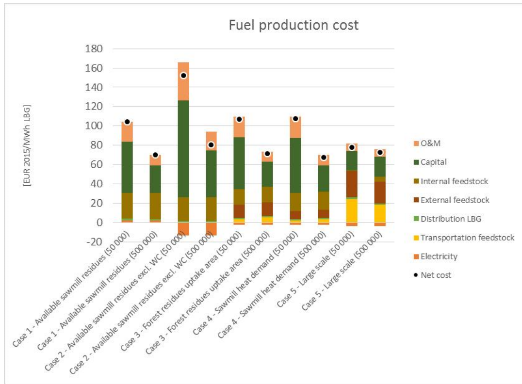
Figure 13. Fuel production cost (FPC) for all cases and the 50 000 and 500 000 m³/a sawmill sizes.
