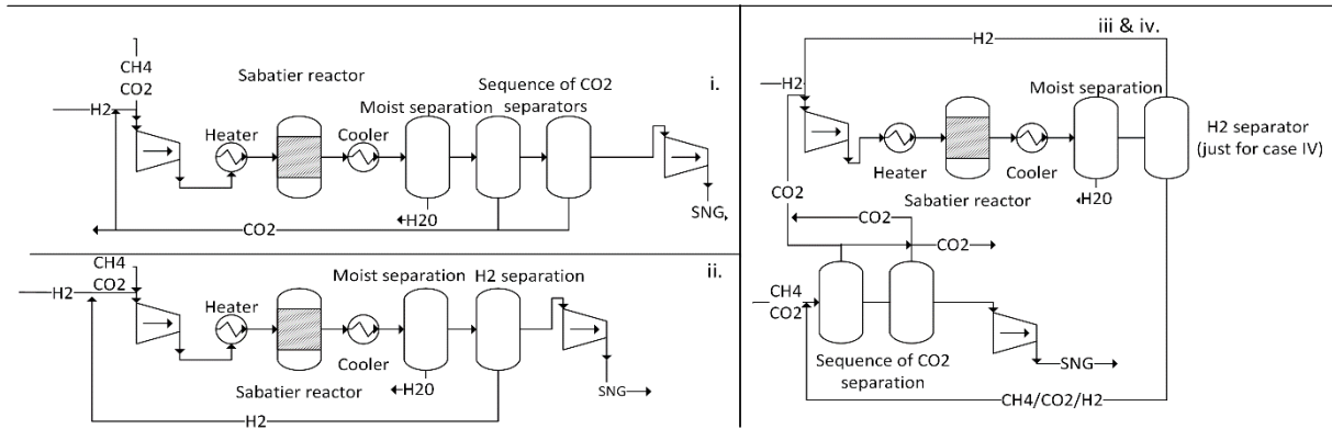
Figure 4. Overview of the final CO 2 removal sequence for the four configurations.
