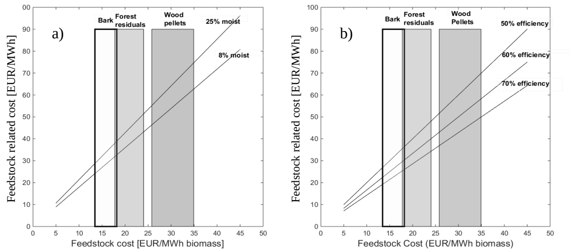
Figure 11. Economic sensitivity analysis. Bars represents feedstock prices with a sensitivity of \pm 15\% ; lines show the feedstock related cost as a function of feedstock cost for different moisture contents (a) and different biomethane efficiencies (b)
