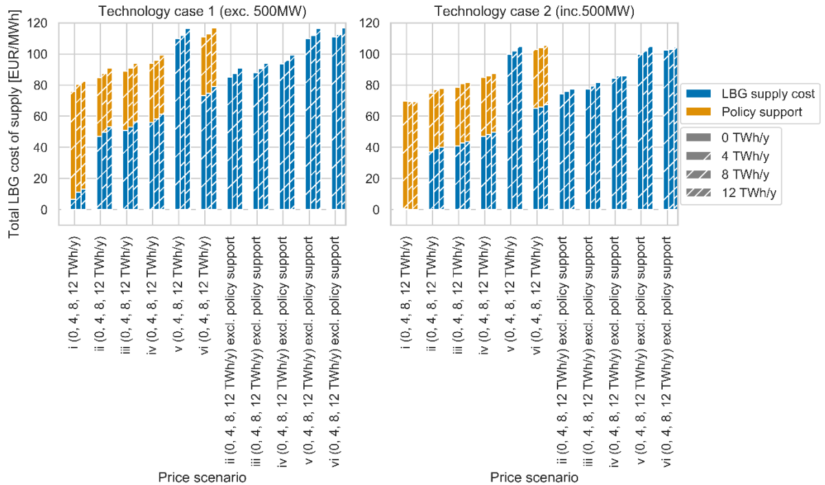
Figure 16. Total system cost of supplying LBG for Technology case 1 (upper) and Technology case 2 (lower).
