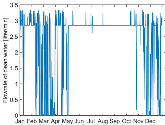
Fig. 17. Flow rate of clean water [liter/min] from desalination powered by two WECs in Kilifi, Kenya, during 2015.
