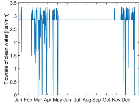
Fig. 18. Flow rate of clean water [liter/min] from desalination powered by three WECs in Kilifi, Kenya, during 2015.
