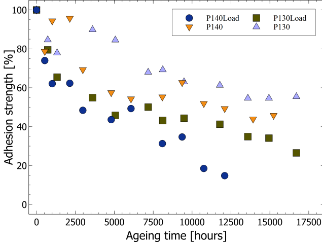
Figure 4.11: Adhesion strength measured on P140, P140Load, P130 and P130Load pipes over two years.
