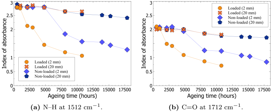
Figure 4.13: Index of absorbance for the peaks at 1512\text{ cm}^{-1} (a) and 1712\text{ cm}^{-1} (b) from P140 and P140Load [Figure 14 in Paper IV].
