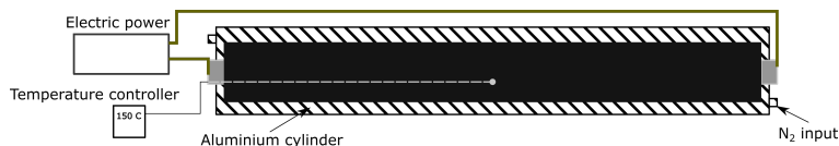
Figure 3.8: Sketch of the test set-up for accelerated ageing of a DH pipe in an inert environment.
