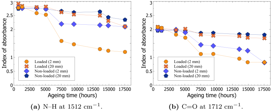
Figure 4.12: Index of absorbance for the peaks at 1512\text{ cm}^{-1} (a) and 1712\text{ cm}^{-1} (b) from P130 and P130Load [Figure 13 in Paper IV].
