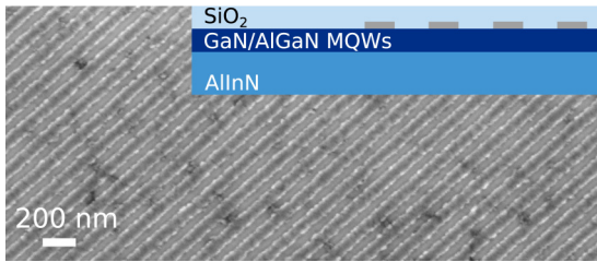
FIG. 10. SEM image of a representative evaporated Al grating after lift-off and before \text{SiO}_2 deposition. Inset: Sketch of the sample structure. Gratings extend over 100 \times 100 \mu\text{m}^2 areas and have a 130 nm period. The Al stripes are 70 nm wide.
