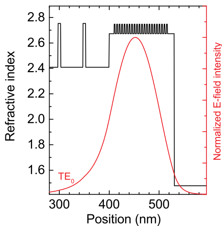
FIG. 11. Optical mode profile along the growth axis, calculated with a finite-difference time-domain mode solver, of the \text{TE}_0 mode supported by the waveguide. The position is measured from the interface between the GaN buffer and the bottom cladding. The refractive index for (Al)GaN is taken from Ref. [51], while the refractive index of AlInN is taken from Ref. [52], and the refractive index of \text{SiO}_2 is issued from experimental data.
