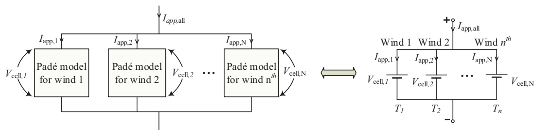
Figure 3. Parallel connection of Padé models.
