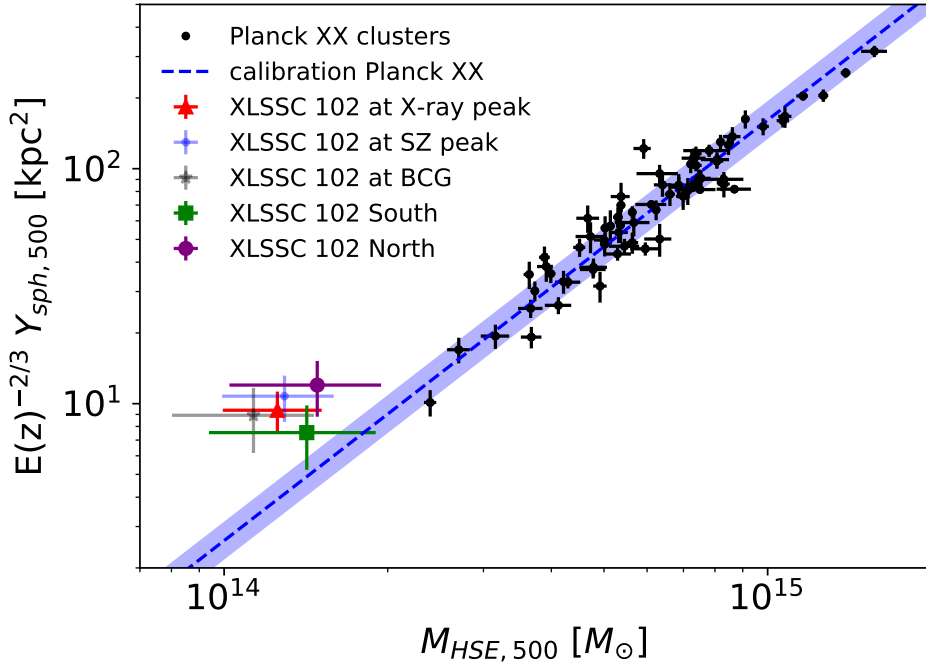
Fig. 11. Location of XLSSC 102 on the scaling relation between the spherically integrated Compton parameter Y_{500} and the hydrostatic mass M_{\text{HSE},500} (i.e. the total mass assuming b_{\text{HSE}} = 0 ). The different markers indicate the values from the combined SZ+X-ray analysis of XLSSC 102 evaluated on the entire cluster at different centres and from the southern and northern regions at the X-ray centre, as indicated in the legend. The values and error bars represent the median and the 68% c.i. The black data points show the Planck calibration cluster sample corrected from Malmquist bias. The blue line and region indicate the fitted relation and its intrinsic scatter ( Planck XX ).
