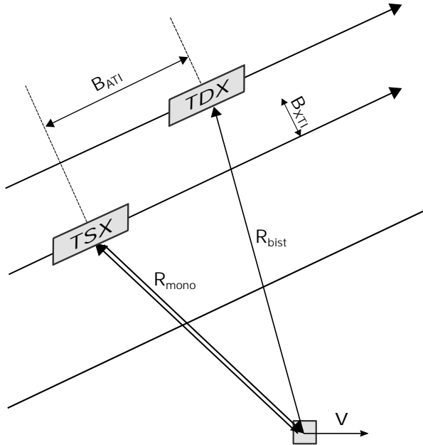
Figure 2.4. TanDEM-X: a hybrid, single-pass and bistatic interferometric SAR.
