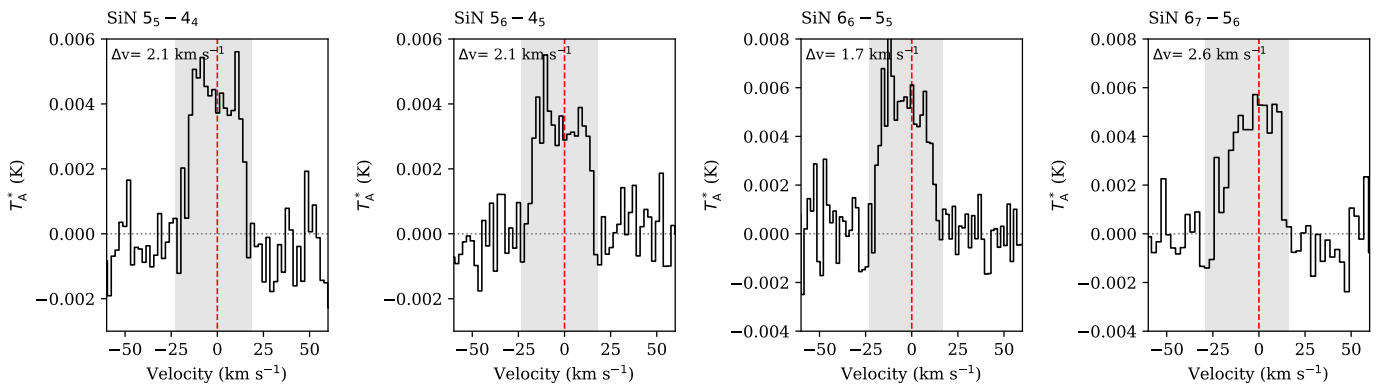
Fig. B.6. SiN emission. Rest frequencies were calculated by weighting the hyperfine component frequencies with the intrinsic component intensities.
