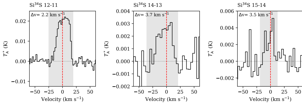
(d) 34 SiS. Note that the J = 12 - 11 emission is blended with emission from 30 SiO ( J = 5 - 4 )
