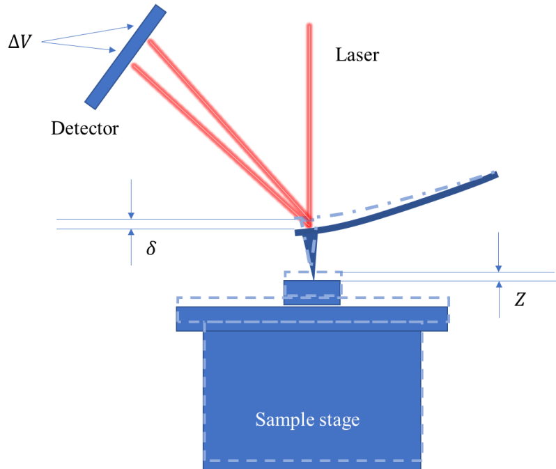
Figure 2. Schematic diagram of atomic force microscopy.
