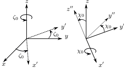
Fig. 1. Two-step rotation: First around z -axis, then around x' -axis, as the rotation angle around the x' -axis. See Fig. 1. This is representative of practical applications characterized by two rotation angles, such as vehicular and robotic applications 1 . Both BS and UE are equipped with antenna arrays of arbitrary but known geometries and communicate through a LOS. In this context, we assume that the NLOS parameters, if any, can be estimated as in [10]. However, unlike [10], we use only the DOA, DOD and TOA of the LOS path to compute the PEB and OEB. Consequently, for clarity, we can write the signal model explicitly by including only the LOS 2 .
