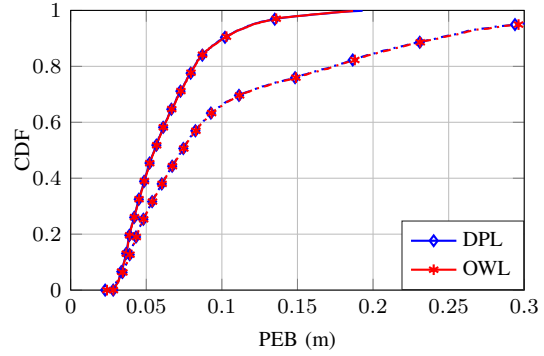
Fig. 3. CDF of PEB with UE orientation angles of 0^\circ (solid) and 15^\circ (dash-dot). N_{\text{U}} = N_{\text{B}} = 144 , N_{\text{B}} = 25 .
