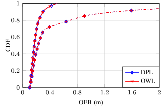
Fig. 4. CDF of OEB with UE orientation angles of 0^\circ (solid) and 15^\circ (dash-dot). N_{\text{U}} = N_{\text{B}} = 144 , N_{\text{B}} = 25 .
