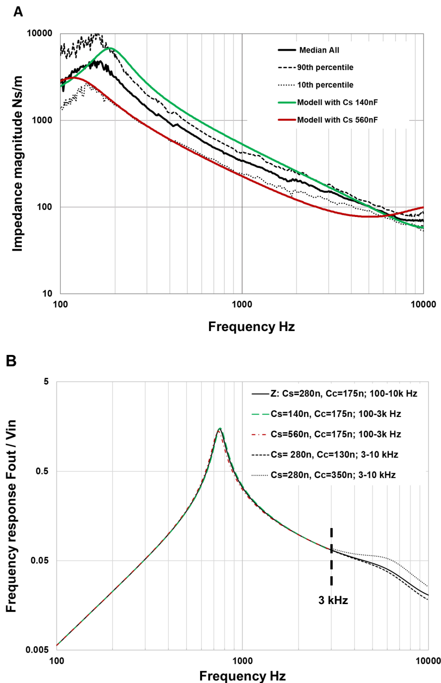
Figure 14 Median, 90th and 10th percentiles of the measured skull impedance magnitudes and the modeled skull impedance magnitudes with extreme values of Cs (A). Magnitudes of the simulated frequency response using the electro-mechanical analogy model of the transducer and modelled impedance (B) where besides nominal values of Cs (280nF) and Cc (175nF) also the extreme values of skull compliance Cs and coupling compliance Cc are used. Note that only Cs is varied below 3k Hz and only Cc is varied above 3k Hz.
