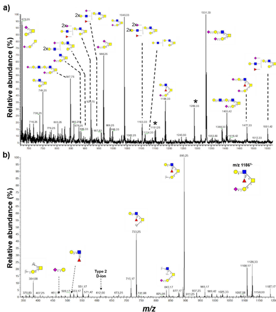
Figure 6. Dominant core 2 O-glycosylation in SG and GG fractions. a , core 2 O-glycans were commonly observed with LacNAc extensions on the 6' arm and sialic acid capping on the 3' arm galactose in SG + GG fractions. b , LC-MS/MS spectra of core 2 O-glycan ( m/z 1186 1- ) with sialic acid capping on the 3' arm and Lewis epitope on the 6' arm. Asterisks represent contaminating signals of unknown origin. Blue squares, GlcNAc; yellow squares, GalNAc; red triangles, fucose; yellow circle, galactose; purple diamonds, sialic acid ( N -acetylneuraminic acid).
