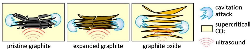
Fig. 4 Illustration of the exfoliation process of pristine graphite, expanded graphite and graphite oxide in ultrasonic-assisted scCO_2 process (reprinted/reproduced with the permission of Ref. [71], copyright 2017, Ultrasonics Sonochemistry)
